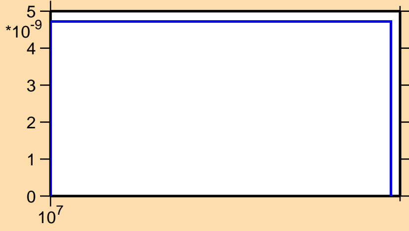
\sigma vs. E for ^{192}\text{Bi}(n,\text{pt})
