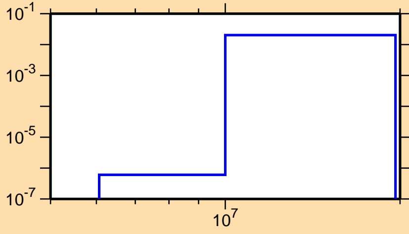
\sigma vs. E for ^{192}\text{Bi}(n,2n\alpha)
