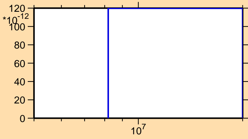
\sigma vs. E for ^{192}\text{Bi}(\text{mt } 34)
