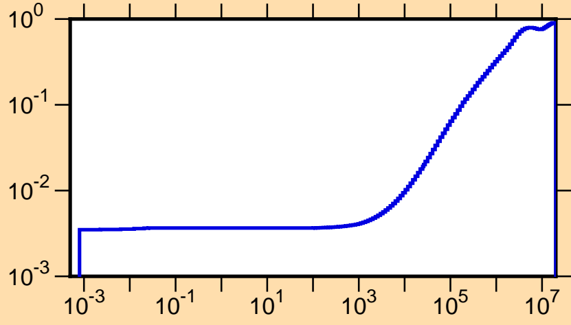
\mu vs. E for ^{193}\text{Bi}(\text{mt251})
