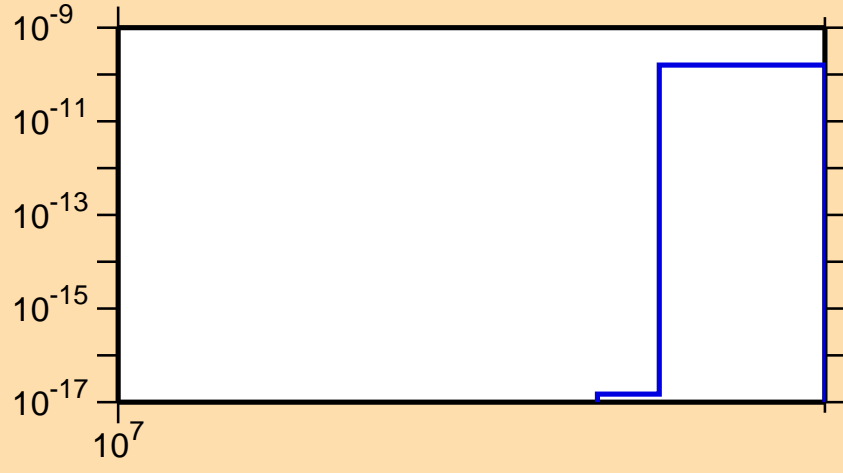
\sigma vs. E for ^{193}\text{Bi}(n,3n\alpha)
