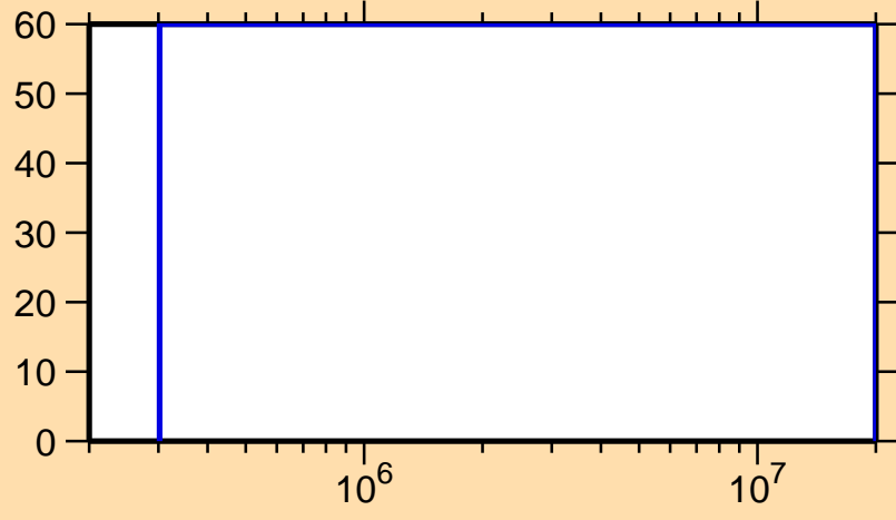
\Delta\sigma/\sigma vs. E for ^{193}\text{Bi}(n,n_1)
