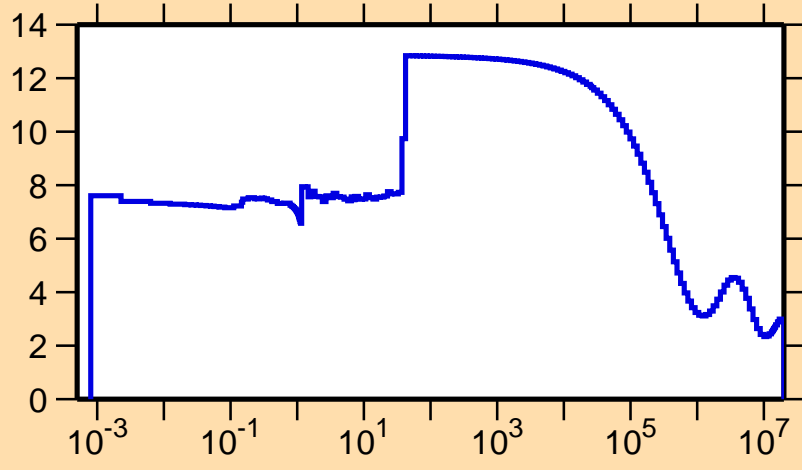
\sigma vs. E for ^{193}\text{Bi}(n,\text{el.})
