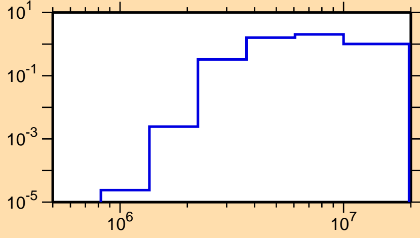
\sigma vs. E for ^{193}\text{Bi}(n,n\text{cont.})
