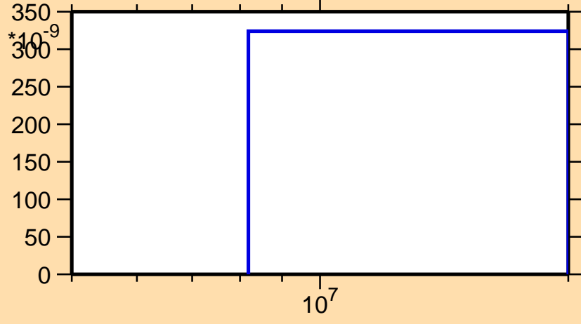
\sigma vs. E for ^{193}\text{Bi}(n,3n)
