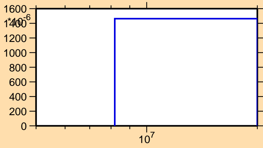
\sigma vs. E for ^{193}\text{Bi}(n,2n\alpha)
