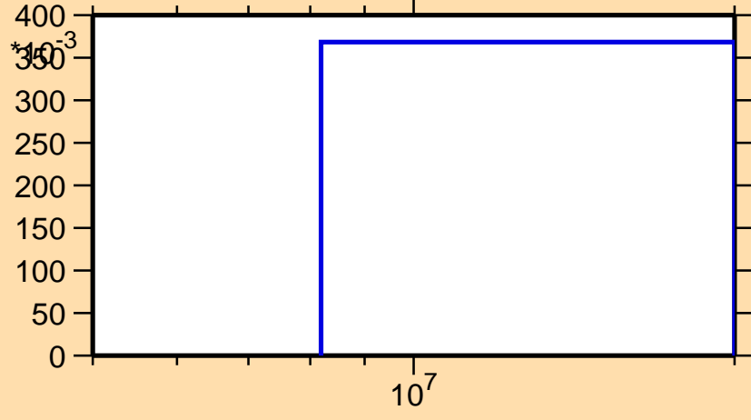
\sigma vs. E for ^{193}\text{Bi}(n,2n)
