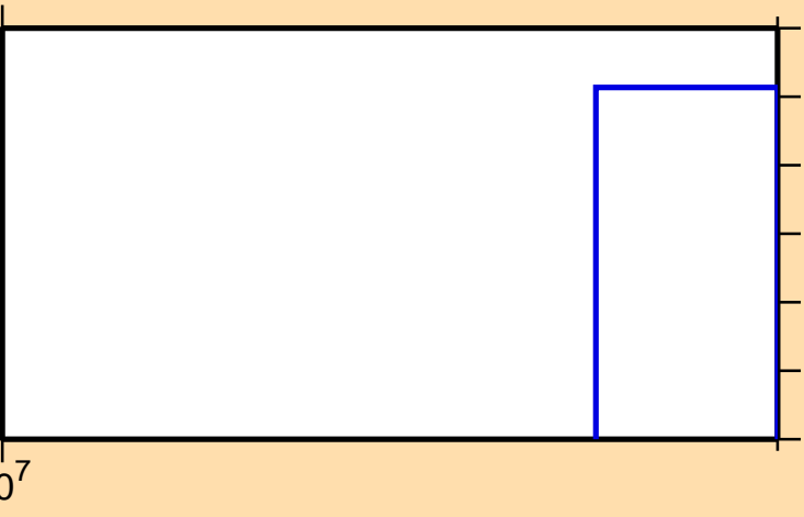
\sigma vs. E for ^{194}\text{Bi}(n,3n)
