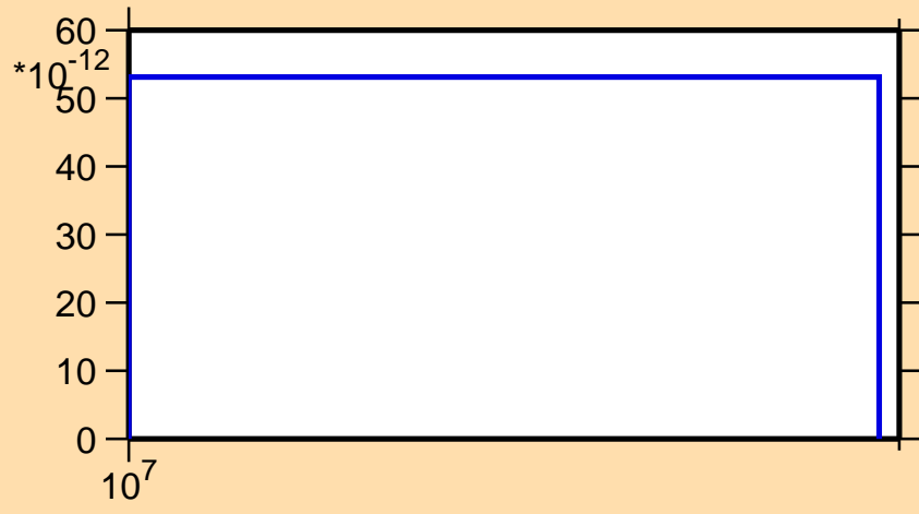
\sigma vs. E for ^{194}\text{Bi}(n,3n\alpha)
