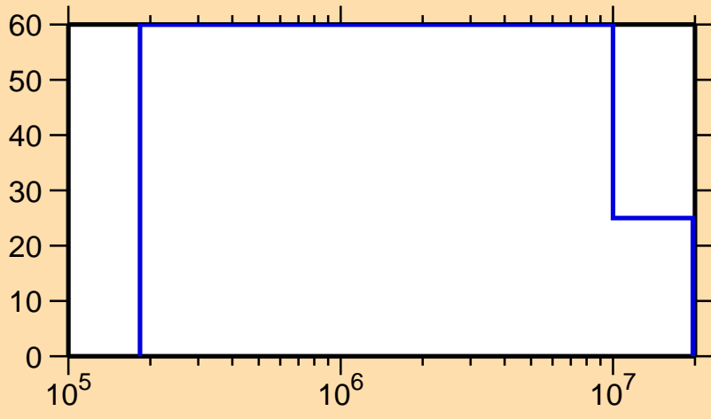
\Delta\sigma/\sigma vs. E for ^{194}\text{Bi}(n,n_1)
