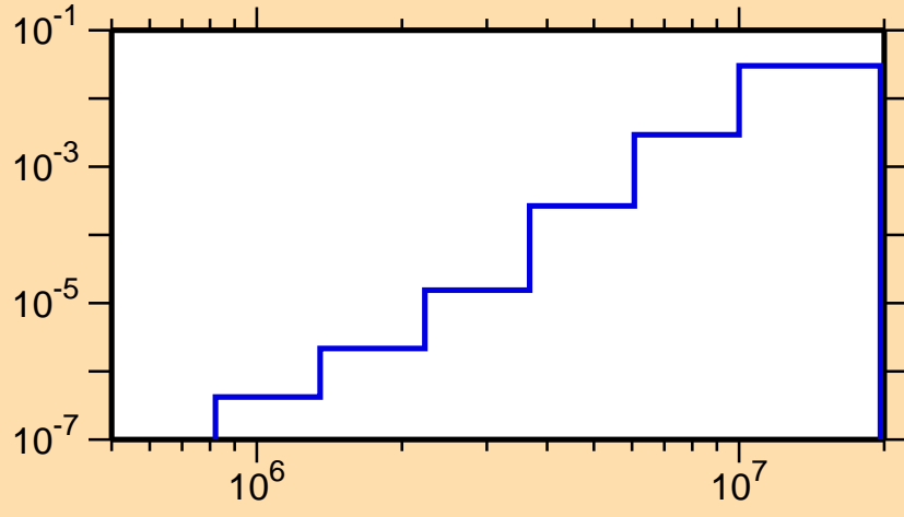
\sigma vs. E for ^{194}\text{Bi}(n,n\alpha)
