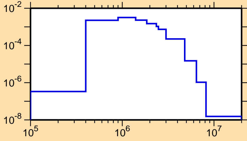
\sigma vs. E for ^{194}\text{Bi}(n,n_4)
