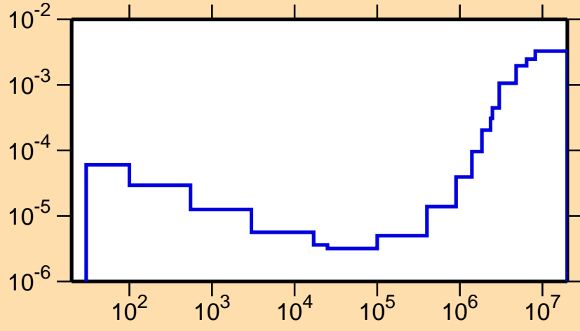
\sigma vs. E for ^{194}\text{Bi}(n,p\alpha)
