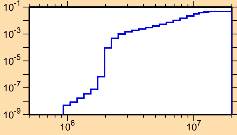
\sigma vs. E for ^{195}\text{Bi}(n,n\alpha)
