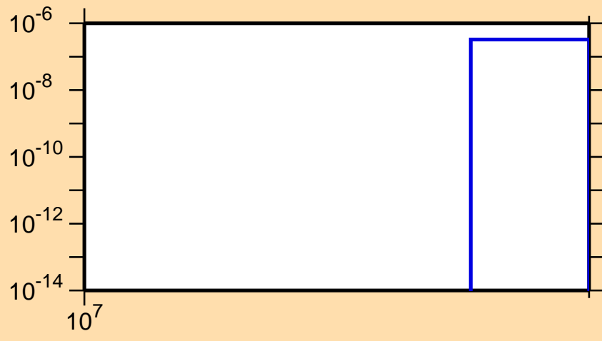
\sigma vs. E for ^{195}\text{Bi}(n,3n\alpha)
