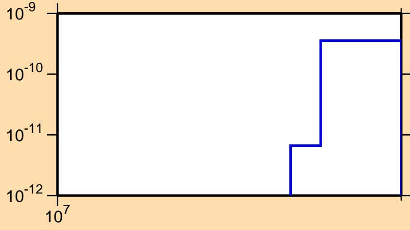
\sigma vs. E for ^{195}\text{Bi}(n,\text{pt})
