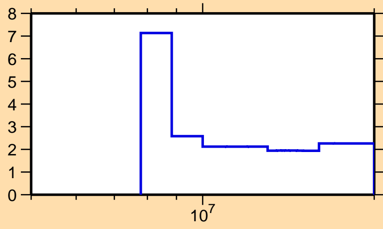
\Delta\sigma/\sigma vs. E for ^{196}\text{Bi}(n,\text{tot.})
