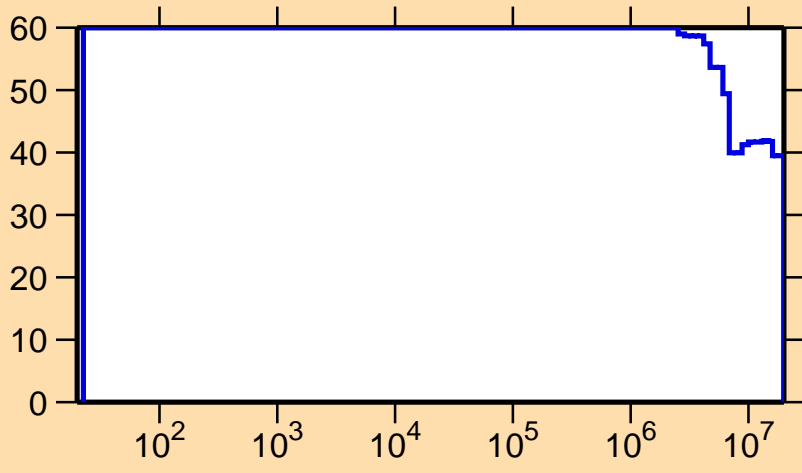
\Delta\sigma/\sigma vs. E for ^{196}\text{Bi}(n,p)
