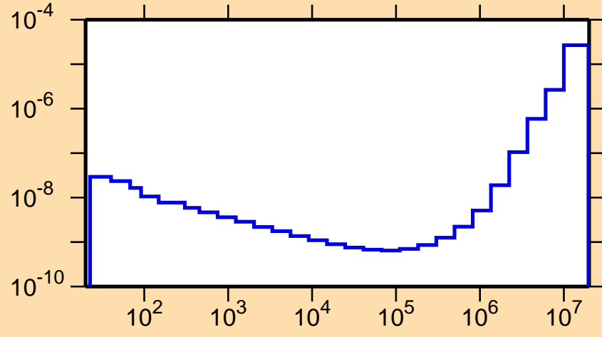
\sigma vs. E for ^{196}\text{Bi}(n,p\alpha)
