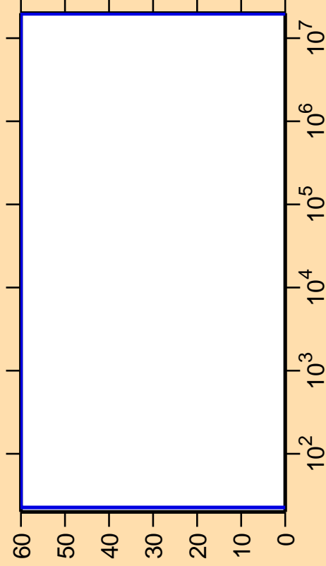
\Delta\sigma/\sigma vs. E for ^{196}\text{Bi}(n,p\alpha)
