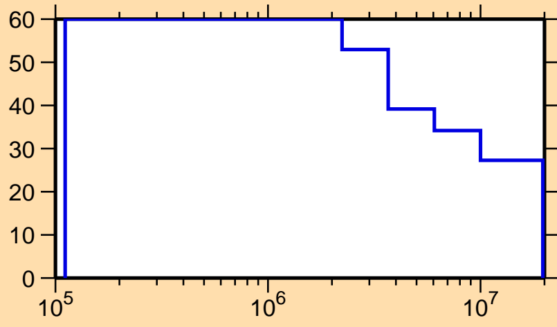
\Delta\sigma/\sigma vs. E for ^{196}\text{Bi}(n,n_1)
