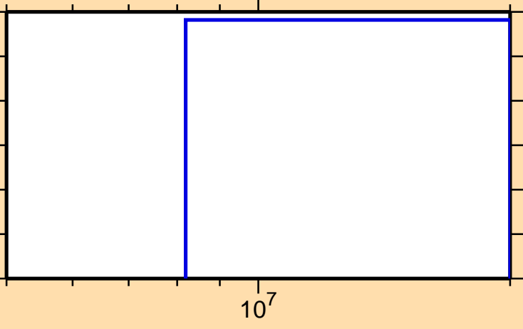
\sigma vs. E for ^{196}\text{Bi}(\text{mt117})
