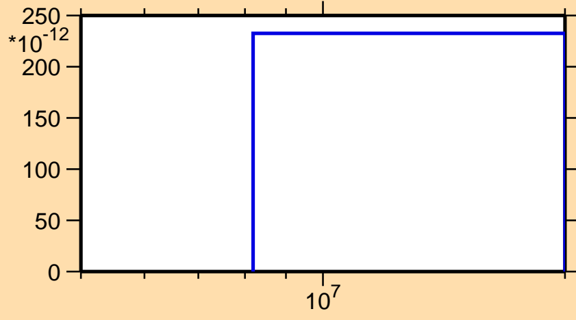
\sigma vs. E for ^{196}\text{Bi}(n,3n\alpha)
