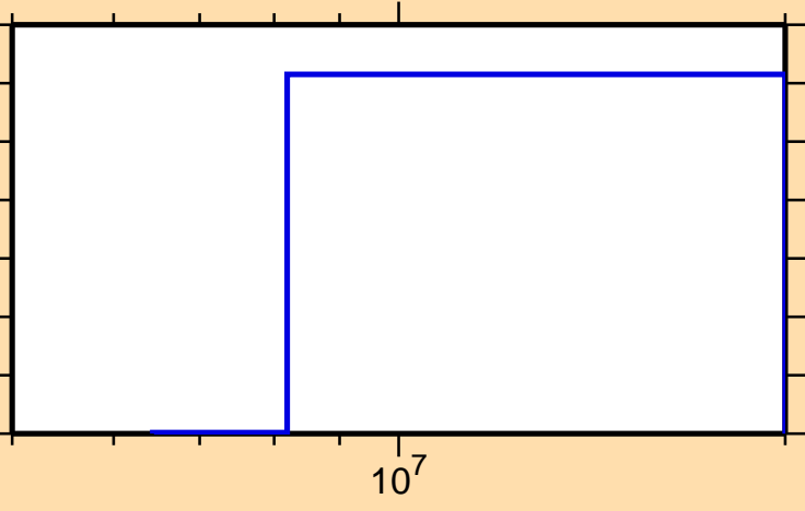
\sigma vs. E for ^{196}\text{Bi}(n,\text{He3})
