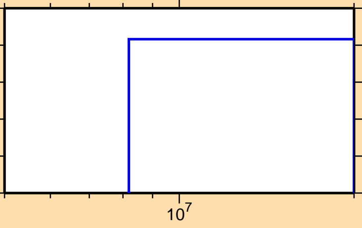
\sigma vs. E for ^{196}\text{Bi}(n,\text{nd})
