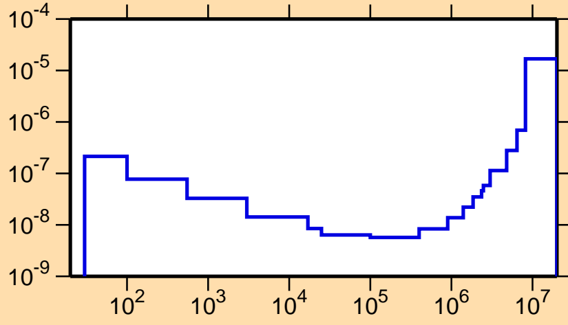
\sigma vs. E for ^{196}\text{Bi}(n,p\alpha)
