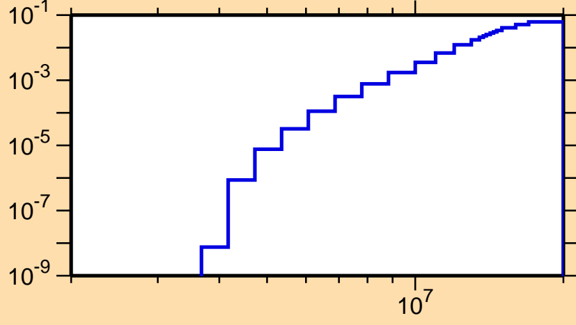
\sigma vs. E for ^{197}\text{Bi}(n,np)
