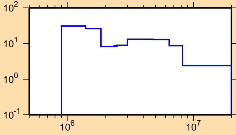
\Delta\sigma/\sigma vs. E for ^{197}\text{Bi}(n,tot.)
