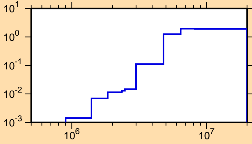
\sigma vs. E for ^{197}\text{Bi}(n,n\text{cont.})
