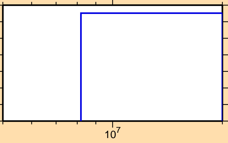
\sigma vs. E for ^{197}\text{Bi} (mt 34)
