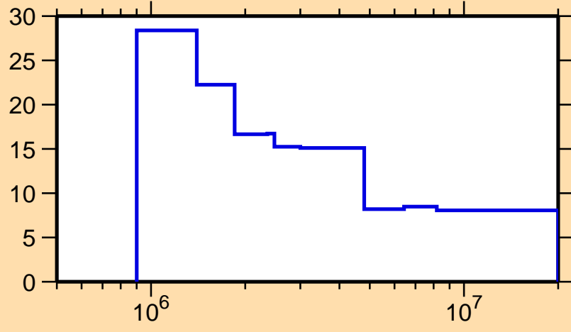
\Delta\sigma/\sigma vs. E for ^{197}\text{Bi}(n,n\text{nonel.})
