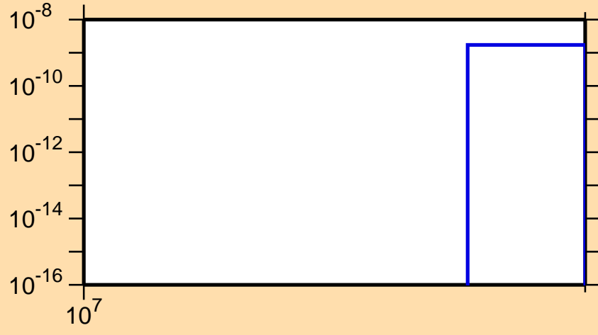
\sigma vs. E for ^{197}\text{Bi}(n,3n\alpha)
