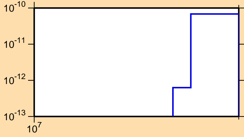
\sigma vs. E for ^{197}\text{Bi}(n,\text{pt})
