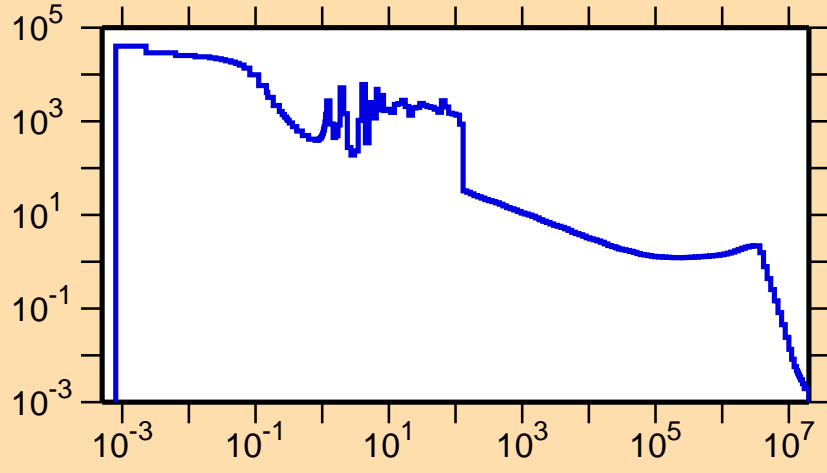
\sigma vs. E for ^{197}\text{Bi}(n,\gamma)
