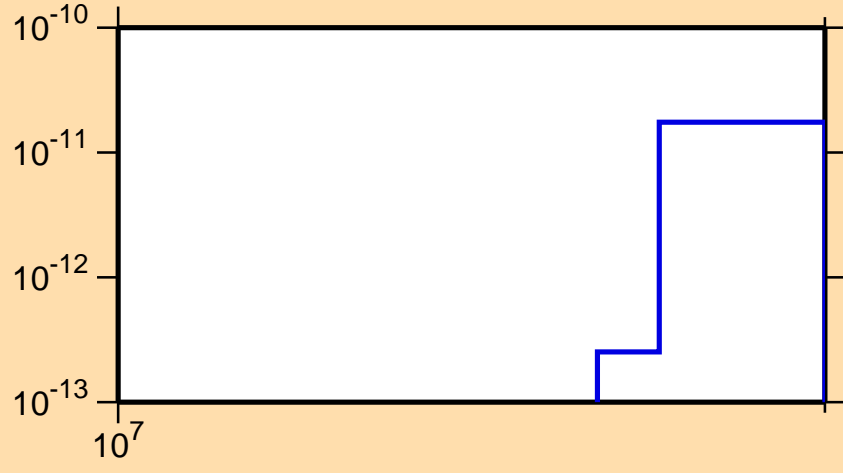
\sigma vs. E for ^{197}\text{Bi} (mt 34)
