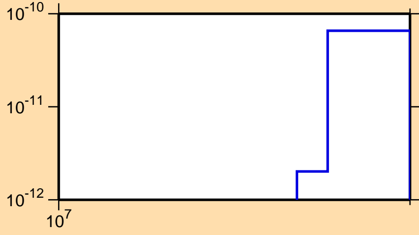
\sigma vs. E for ^{198}\text{Bi} (mt 34)
