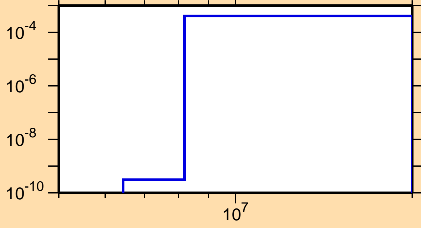
\sigma vs. E for ^{198}\text{Bi}(n,t)
