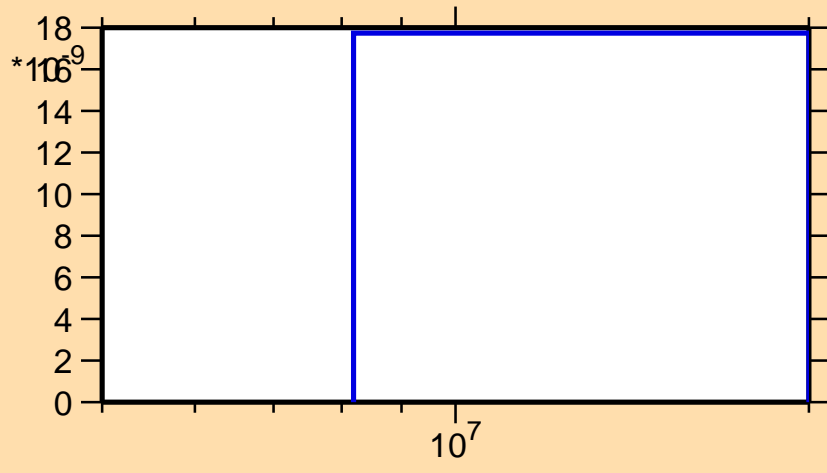
\sigma vs. E for ^{198}\text{Bi} (mt 45)
