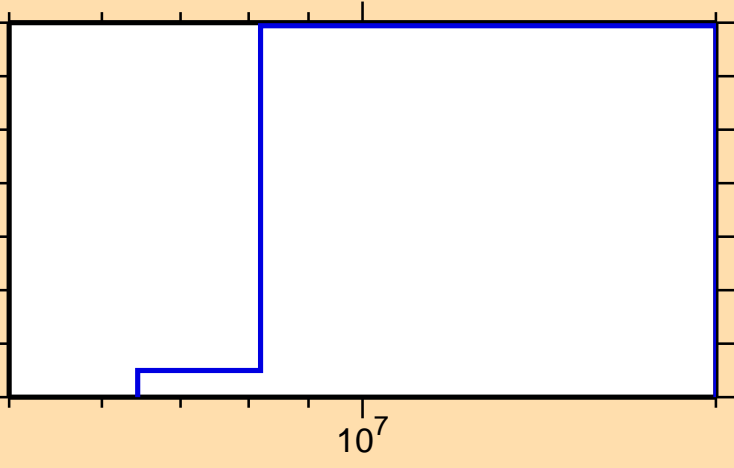
\sigma vs. E for ^{198}\text{Bi}(n,\text{He3})
