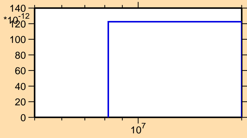
\sigma vs. E for ^{198}\text{Bi}(n,\text{pd})
