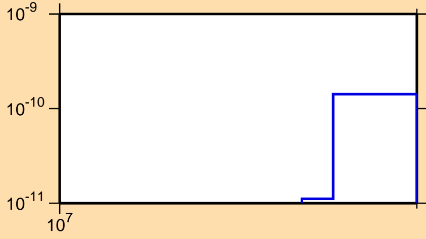
\sigma vs. E for ^{199}\text{Bi}(n,\text{pd})
