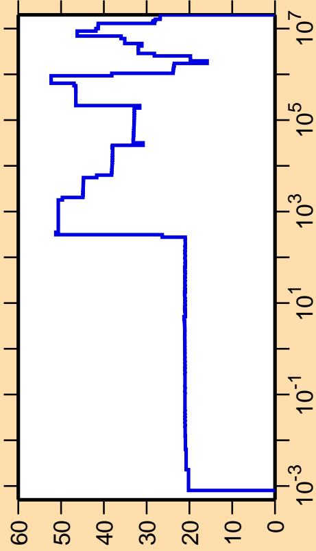
\Delta\sigma/\sigma vs. E for ^{199}\text{Bi}(n,\text{el.})
