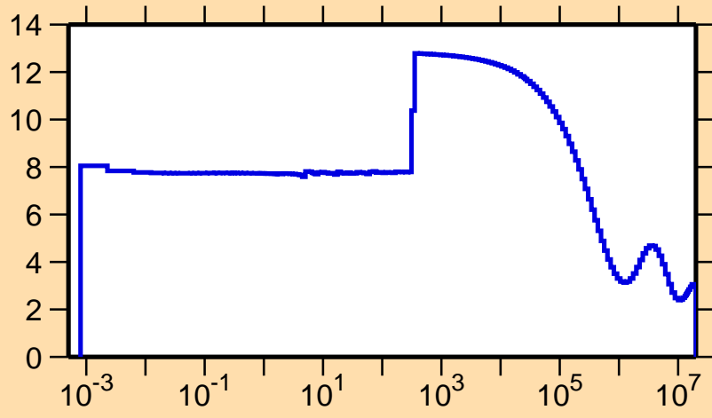
\sigma vs. E for ^{199}\text{Bi}(n,\text{el.})
