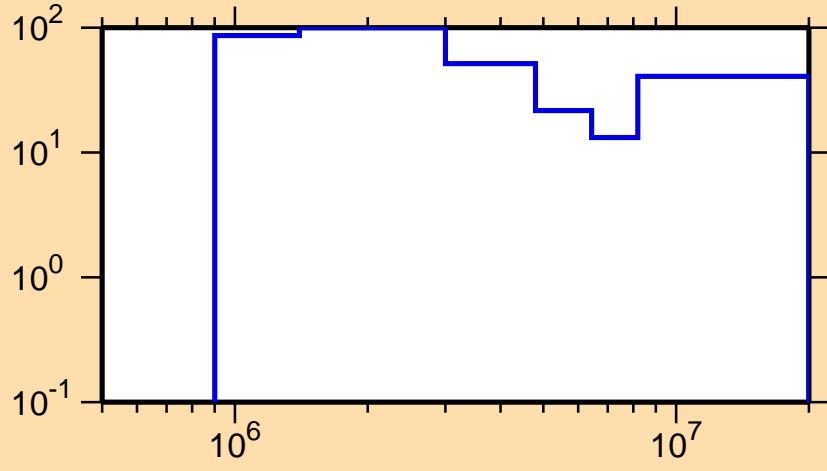
\Delta\sigma/\sigma vs. E for ^{199}\text{Bi}(n,n\text{cont.})
