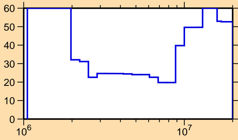
\Delta\sigma/\sigma vs. E for ^{199}\text{Bi}(n,n\text{cont.})
