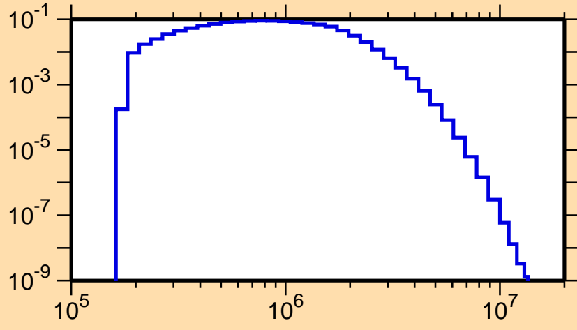
\sigma vs. E for ^{199}\text{Bi}(n,n_2)
