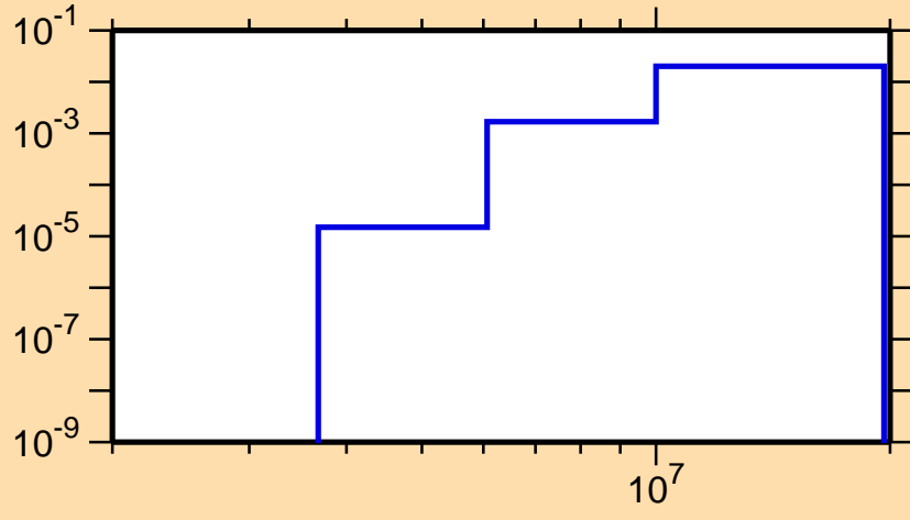
\sigma vs. E for ^{199}\text{Bi}(n,np)
