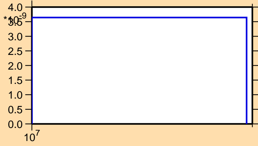
\sigma vs. E for ^{199}\text{Bi}(n,nt)
