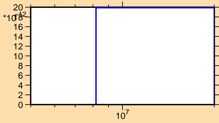
\sigma vs. E for ^{199}\text{Bi}(n,3n\alpha)
