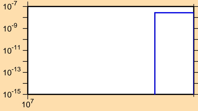
\sigma vs. E for ^{200}\text{Bi}(n,3n\alpha)
