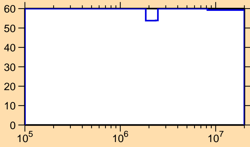
\Delta\sigma/\sigma vs. E for ^{200}\text{Bi}(n,n_1)
