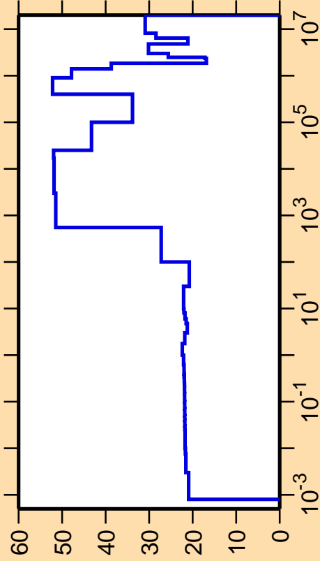
\Delta\sigma/\sigma vs. E for ^{200}\text{Bi}(n,\text{el.})
