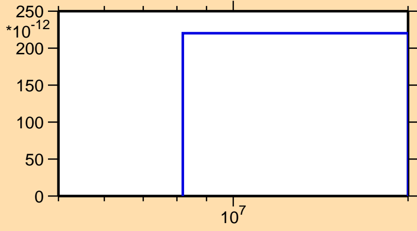
\sigma vs. E for ^{200}\text{Bi}(n,3n\alpha)
