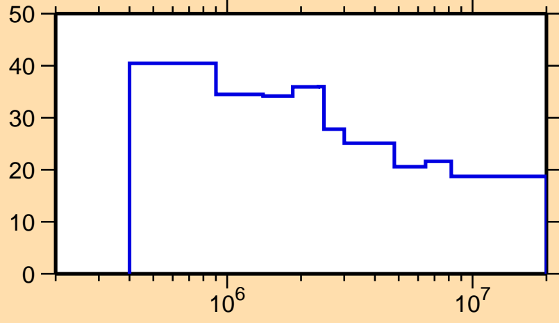
\Delta\sigma/\sigma vs. E for ^{200}\text{Bi}(n,n\text{onel.})
