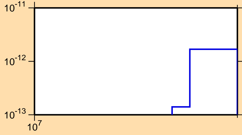
\sigma vs. E for ^{201}\text{Bi}(n,\text{pd})
