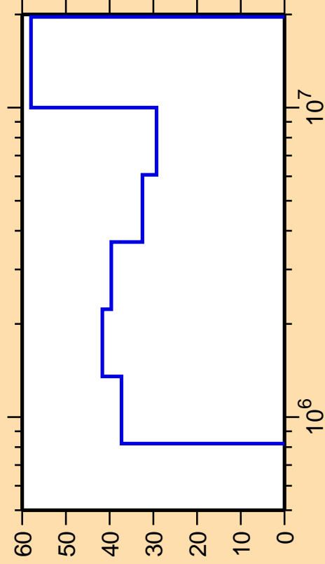
\Delta\sigma/\sigma vs. E for ^{201}\text{Bi}(n,\text{inel.})
