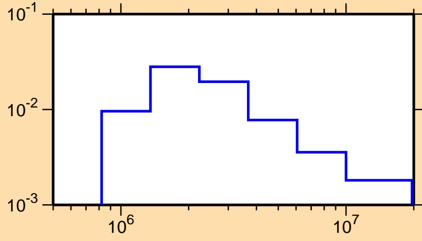
\sigma vs. E for ^{201}\text{Bi}(n,n_4)
