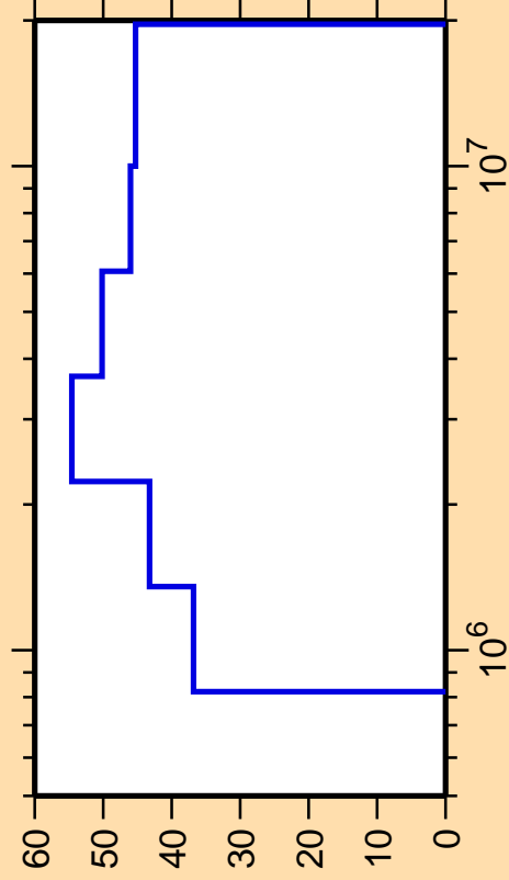
\Delta\sigma/\sigma vs. E for ^{201}\text{Bi}(n,n_4)
