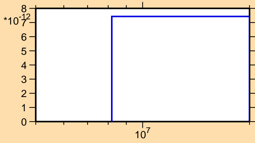
\sigma vs. E for ^{201}\text{Bi}(n,3n\alpha)
