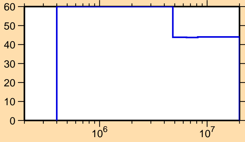
\Delta\sigma/\sigma vs. E for ^{201}\text{Bi}(n,n_1)
