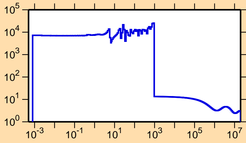
\sigma vs. E for ^{201}\text{Bi}(n,\text{el.})
