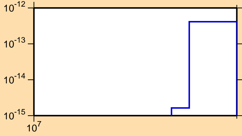
\sigma vs. E for ^{201}\text{Bi}(n,\text{pt})
