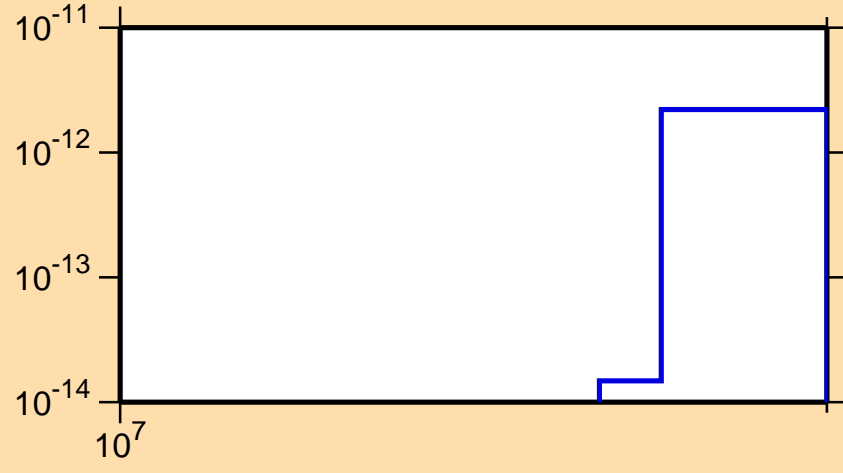
\sigma vs. E for ^{201}\text{Bi} (mt 34)
