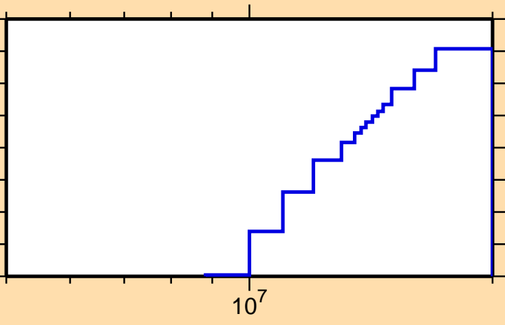
\sigma vs. E for ^{201}\text{Bi}(n,\text{He3})
