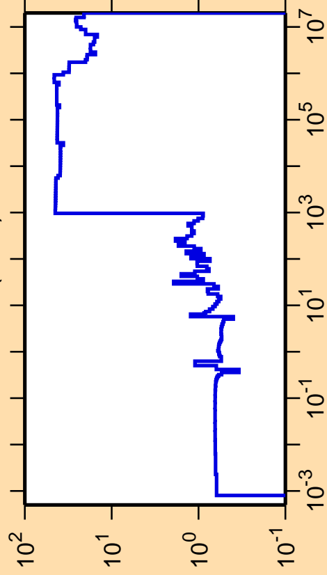
\Delta\sigma/\sigma vs. E for ^{201}\text{Bi}(n,\text{el.})
