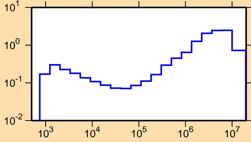
\sigma vs. E for ^{201}\text{Bi}(n,\text{inel.})
