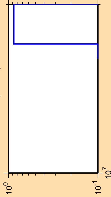
\Delta\sigma/\sigma vs. E for ^{202}\text{Bi}(n,3n\alpha)
