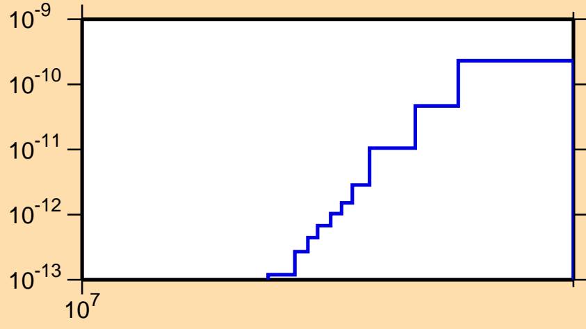
\sigma vs. E for ^{202}\text{Bi}(\text{mt117})
