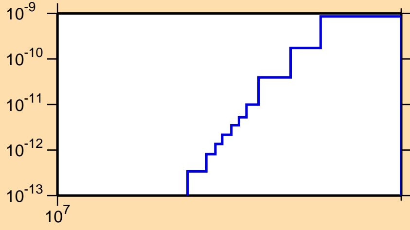
\sigma vs. E for ^{202}\text{Bi} (mt 45)
