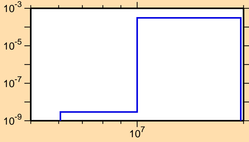
\sigma vs. E for ^{202}\text{Bi}(n,t)
