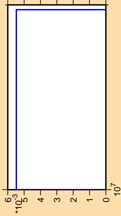
\Delta\sigma/\sigma vs. E for ^{202}\text{Bi}(n,3n\alpha)
