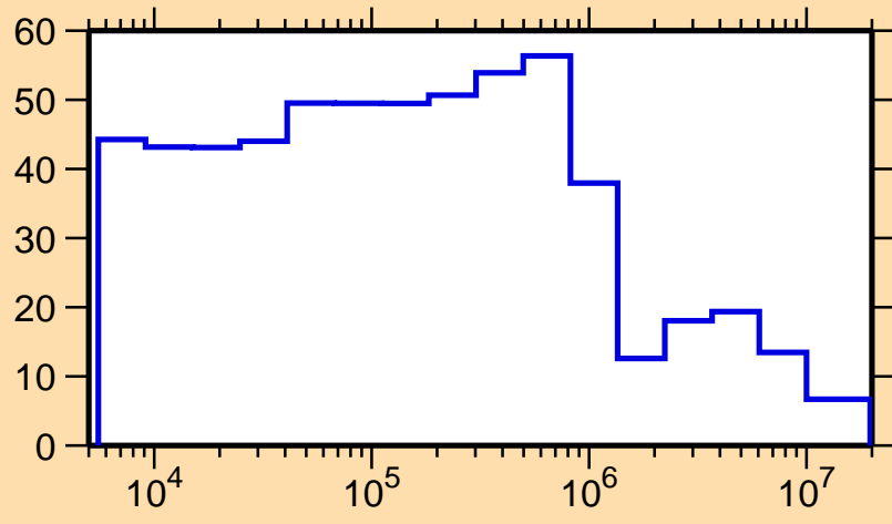
\Delta\sigma/\sigma vs. E for ^{202}\text{Bi}(n,\text{tot.})
