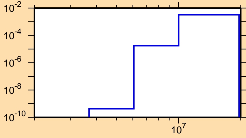
\sigma vs. E for ^{202}\text{Bi}(n,np)
