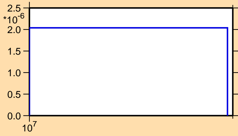
\sigma vs. E for ^{202}\text{Bi}(n,2np)
