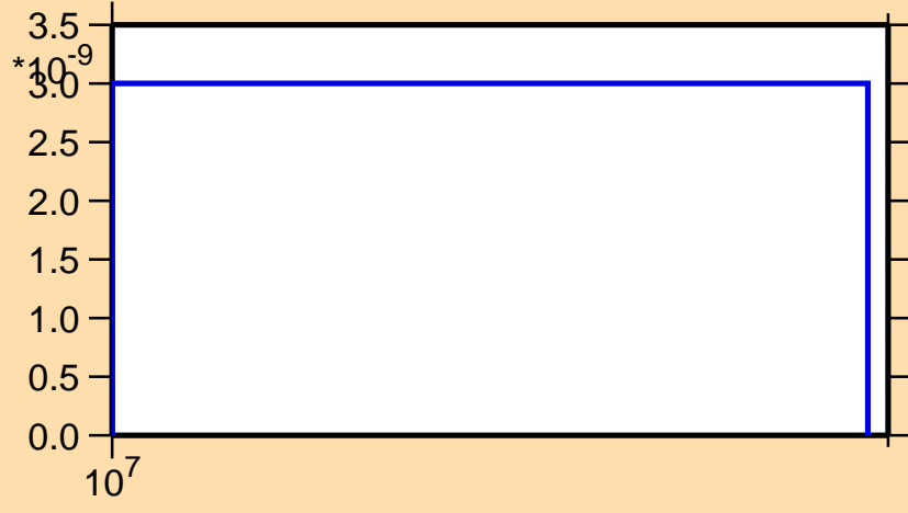
\sigma vs. E for ^{202}\text{Bi}(n,nt)
