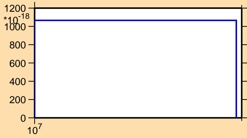
\sigma vs. E for ^{202}\text{Bi}(n,3n\alpha)
