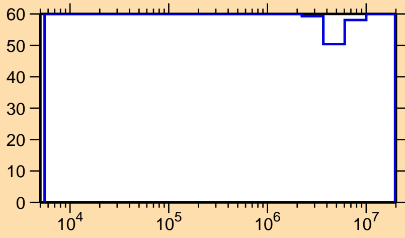
\Delta\sigma/\sigma vs. E for ^{202}\text{Bi}(n,n_1)
