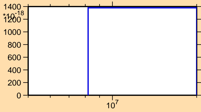
\sigma vs. E for ^{202}\text{Bi}(n,3n\alpha)
