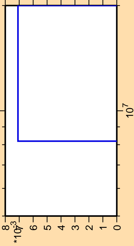
\Delta\sigma/\sigma vs. E for ^{202}\text{Bi}(n,3n\alpha)
