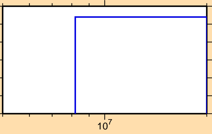
\sigma vs. E for ^{202}\text{Bi}(\text{mt117})
