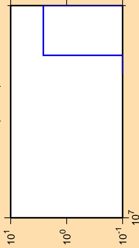
\Delta\sigma/\sigma vs. E for ^{203}\text{Bi}(n,3n\alpha)
