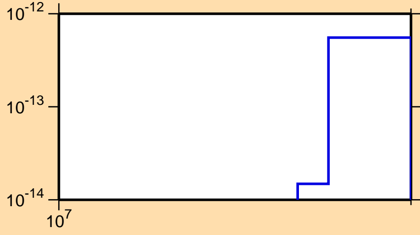
\sigma vs. E for ^{203}\text{Bi}(n,3n\alpha)
