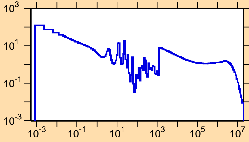
\sigma vs. E for ^{203}\text{Bi}(n,\gamma)
