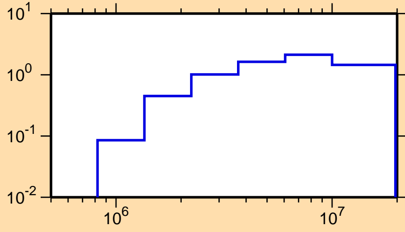
\sigma vs. E for ^{203}\text{Bi}(n,\text{inel.})
