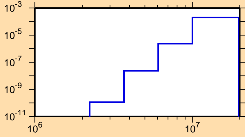
\sigma vs. E for ^{203}\text{Bi}(n,n\alpha)
