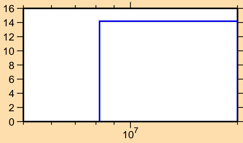
\Delta\sigma/\sigma vs. E for ^{203}\text{Bi}(n,\text{nonel.})
