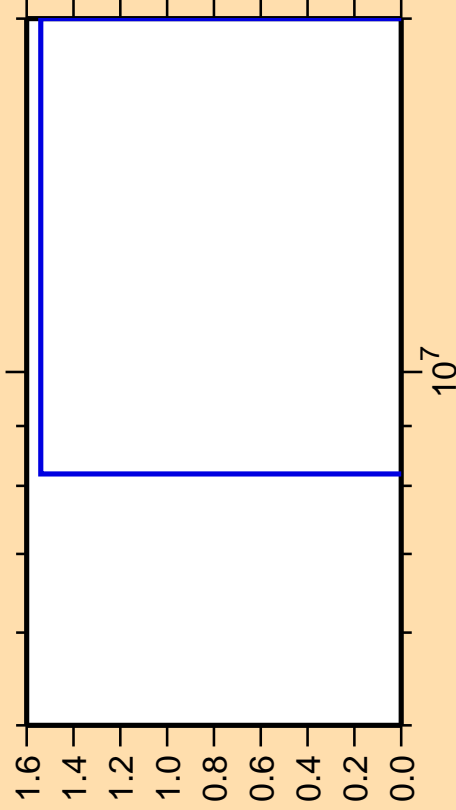
\Delta\sigma/\sigma vs. E for ^{203}\text{Bi}(\text{mt117})
