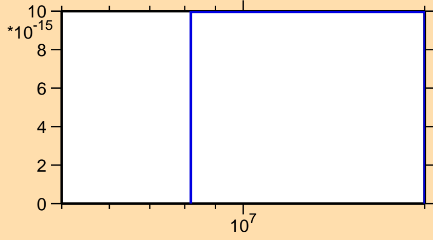
\sigma vs. E for ^{203}\text{Bi}(n,3n\alpha)
