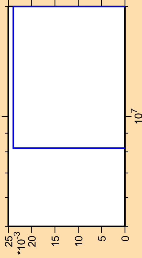
\Delta\sigma/\sigma vs. E for ^{203}\text{Bi}(n,3n\alpha)
