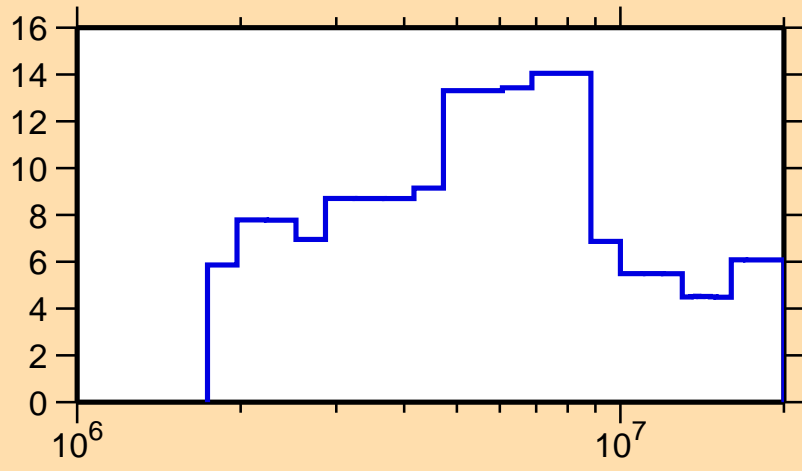
\Delta\sigma/\sigma vs. E for ^{204}\text{Bi}(n,\text{tot.})
