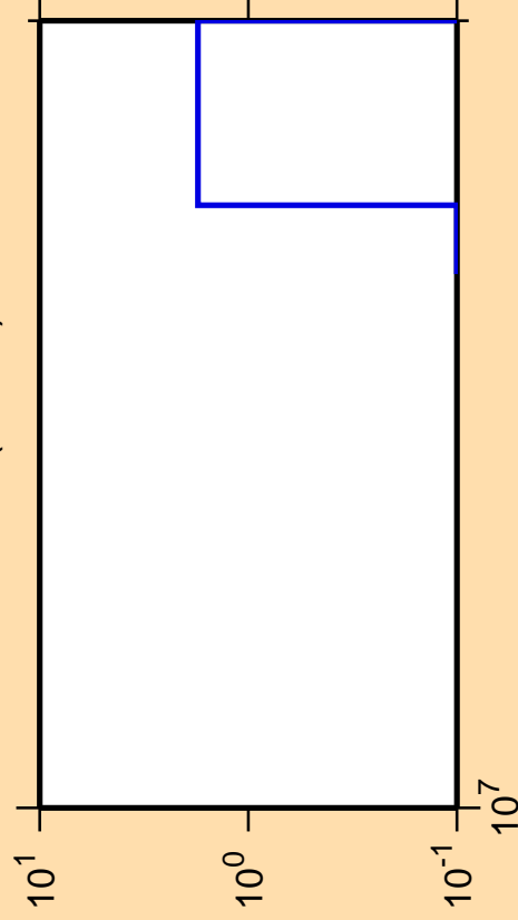
\Delta\sigma/\sigma vs. E for ^{204}\text{Bi} (mt 34)
