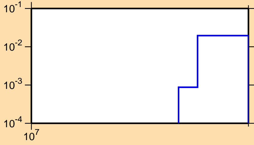
\sigma vs. E for ^{204}\text{Bi}(n,3n)
