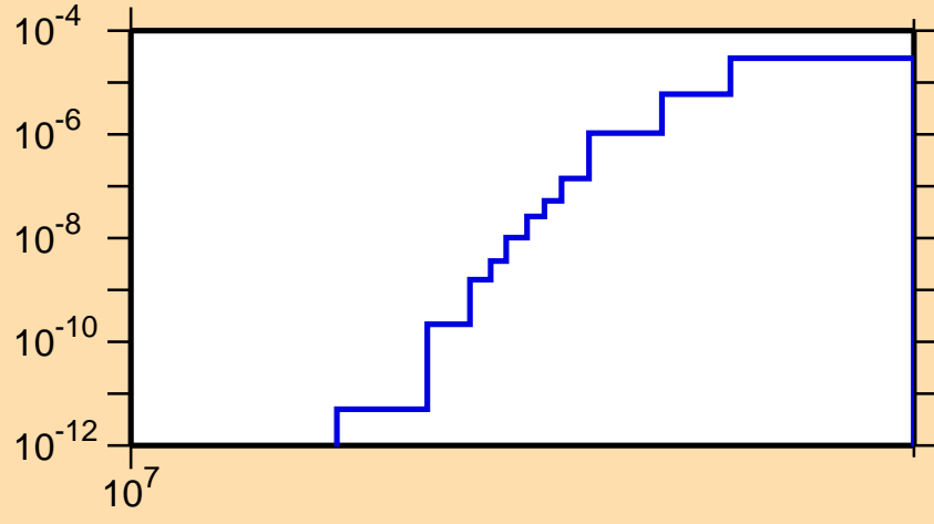
\sigma vs. E for ^{204}\text{Bi}(n,2np)
