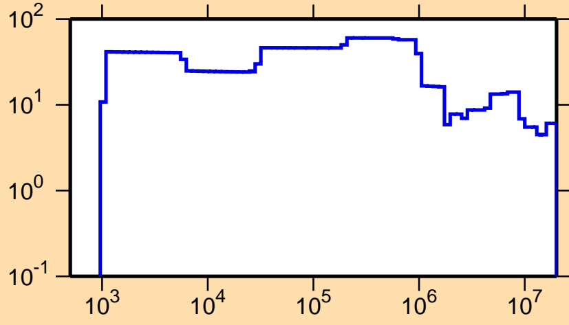
\Delta\sigma/\sigma vs. E for ^{204}\text{Bi}(n,\text{tot.})
