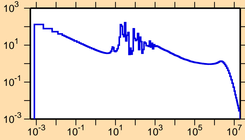
\sigma vs. E for ^{204}\text{Bi}(n,\gamma)
