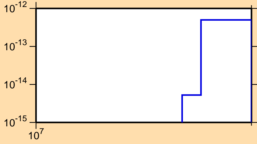
\sigma vs. E for ^{204}\text{Bi}(n,\text{pd})
