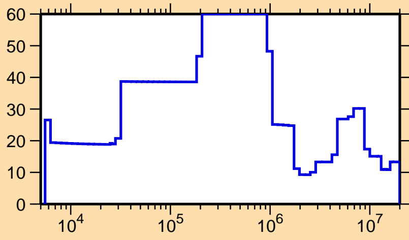
\Delta\sigma/\sigma vs. E for ^{204}\text{Bi}(n,\text{el.})
