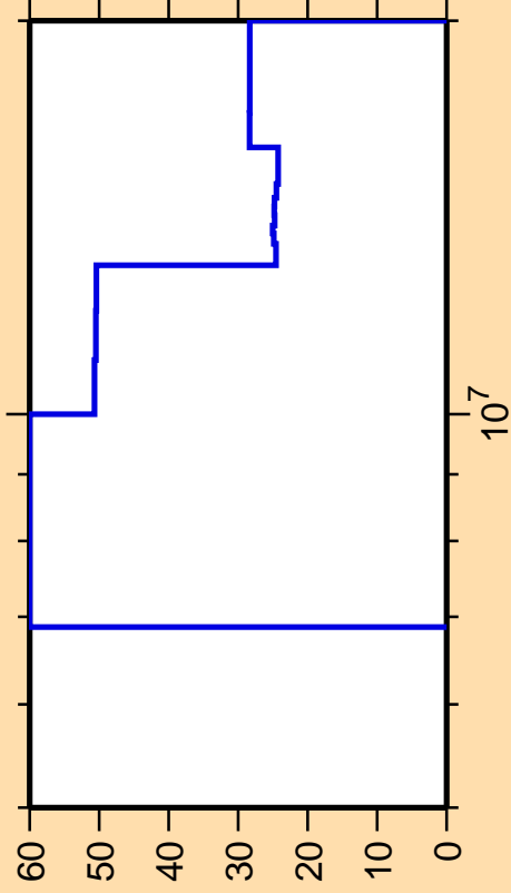
\Delta\sigma/\sigma vs. E for ^{204}\text{Bi}(n,2n)
