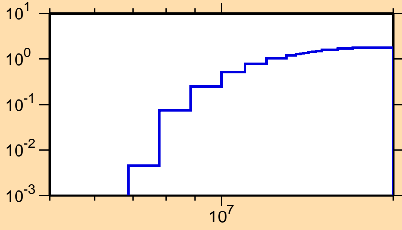
\sigma vs. E for ^{204}\text{Bi}(n,2n)
