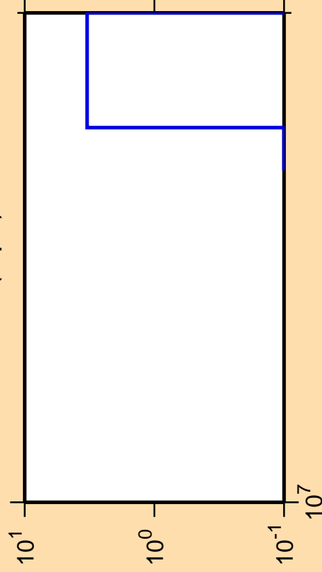
\Delta\sigma/\sigma vs. E for ^{204}\text{Bi}(n,\text{pd})
