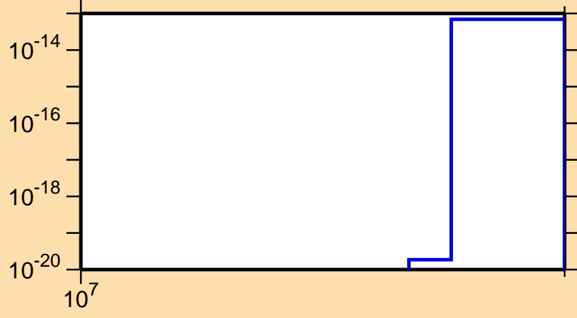
\sigma vs. E for ^{204}\text{Bi}(n,3n\alpha)
