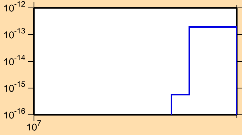
\sigma vs. E for ^{204}\text{Bi} (mt 34)
