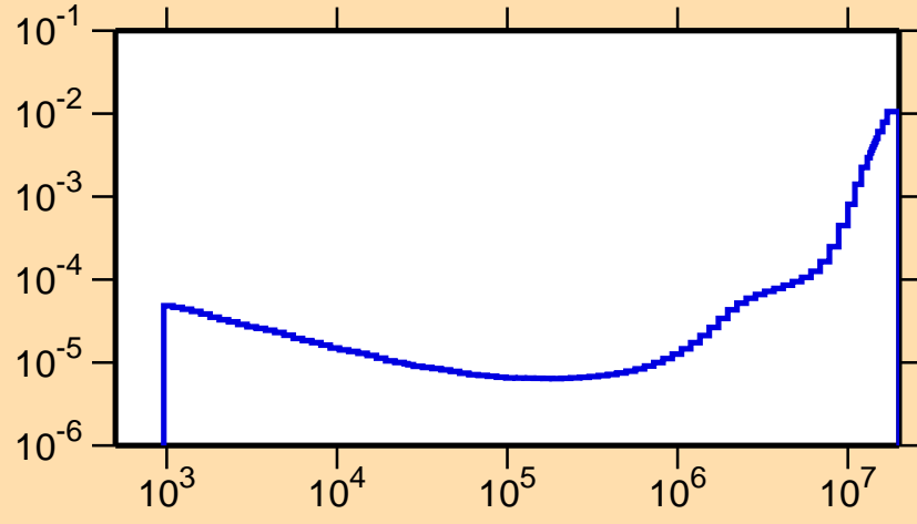
\sigma vs. E for ^{204}\text{Bi}(n,\alpha)
