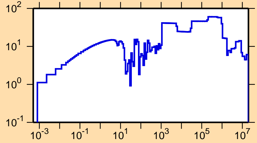
\Delta\sigma/\sigma vs. E for ^{204}\text{Bi}(n,\text{tot.})
