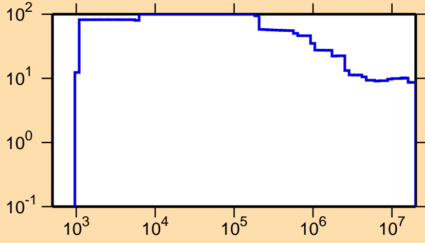
\Delta\sigma/\sigma vs. E for ^{204}\text{Bi}(n,\text{nonel.})
