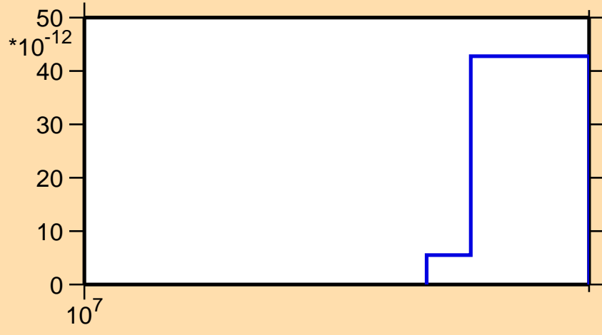
\sigma vs. E for ^{204}\text{Bi} (mt 45)
