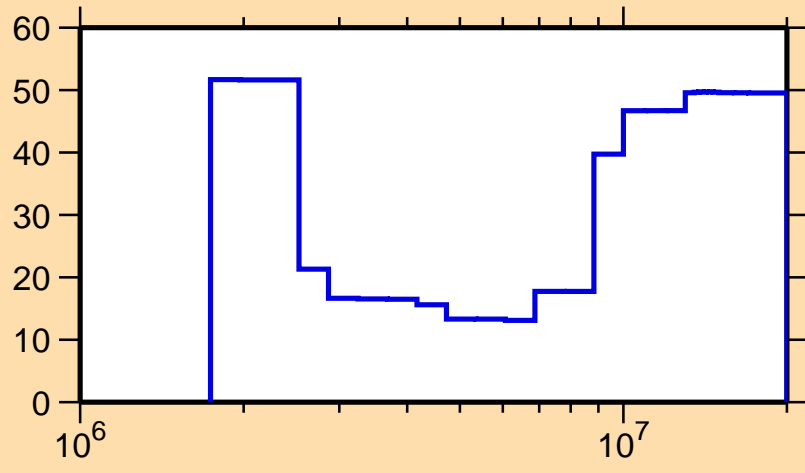
\Delta\sigma/\sigma vs. E for ^{204}\text{Bi}(n,n\text{cont.})
