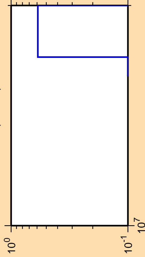
\Delta\sigma/\sigma vs. E for ^{204}\text{Bi}(n,3n\alpha)
