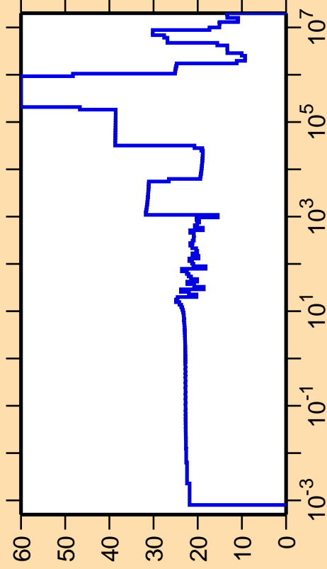
\Delta\sigma/\sigma vs. E for ^{204}\text{Bi}(n,\text{el.})
