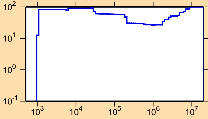
\Delta\sigma/\sigma vs. E for ^{204}\text{Bi}(n,\gamma)
