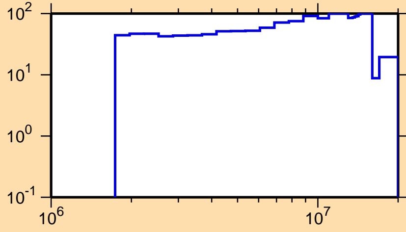
\Delta\sigma/\sigma vs. E for ^{204}\text{Bi}(n,n_1)
