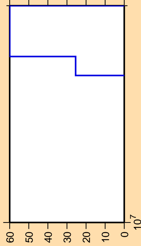
\Delta\sigma/\sigma vs. E for ^{204}\text{Bi}(\text{mt117})
