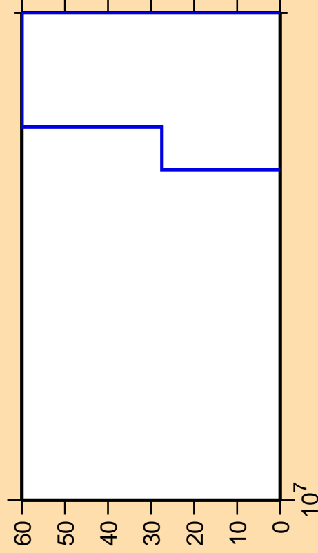
\Delta\sigma/\sigma vs. E for ^{204}\text{Bi} (mt 45)
