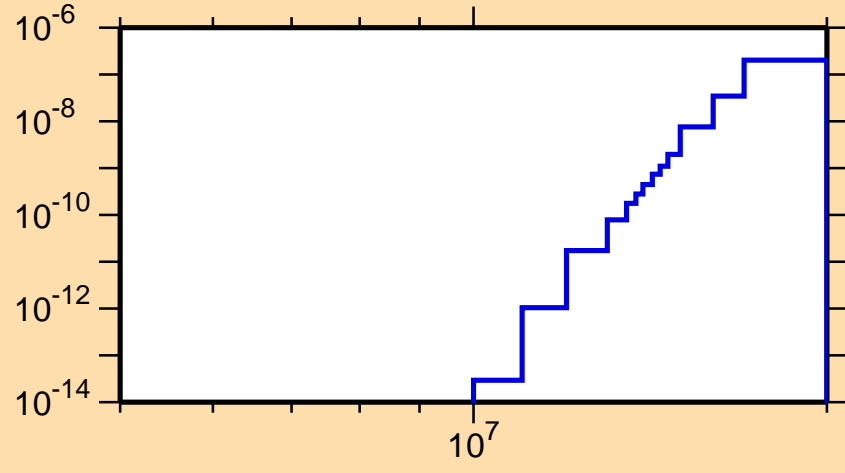
\sigma vs. E for ^{204}\text{Bi}(n,\text{He3})
