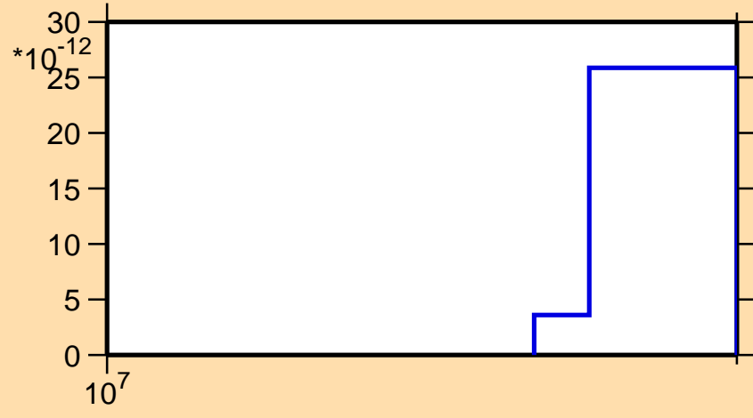
\sigma vs. E for ^{204}\text{Bi}(\text{mt117})
