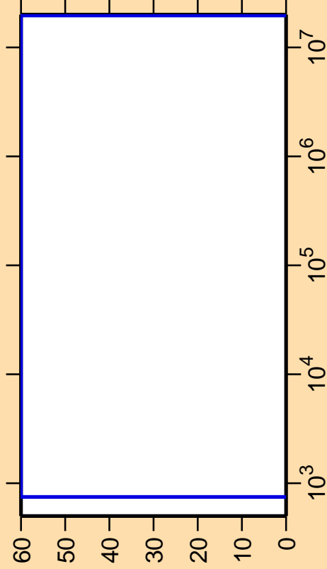
\Delta\sigma/\sigma vs. E for ^{204}\text{Bi}(n,\alpha)
