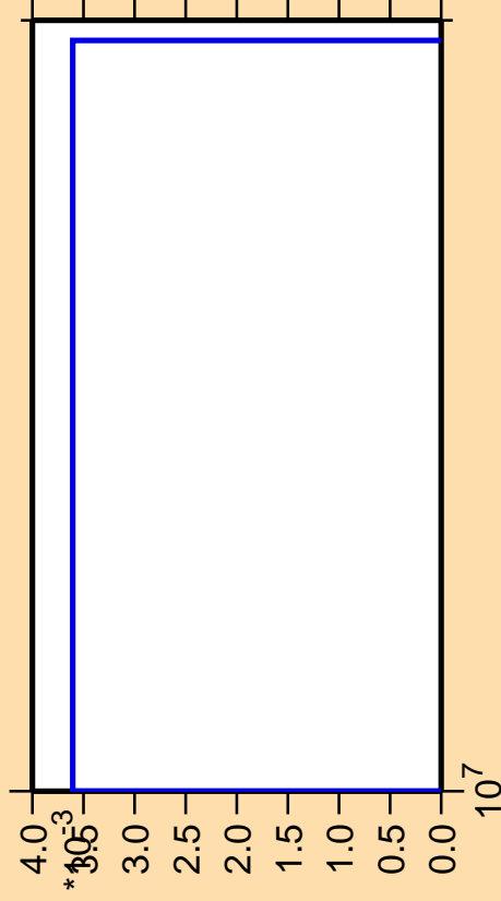
\Delta\sigma/\sigma vs. E for ^{204}\text{Bi}(n,3n\alpha)
