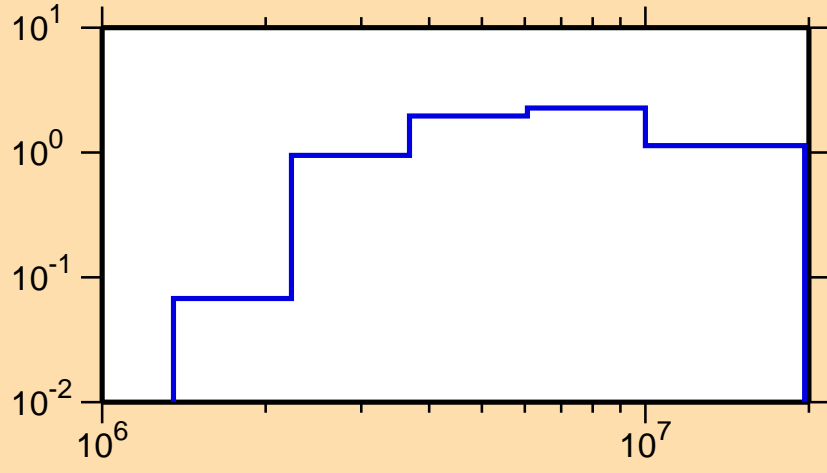
\sigma vs. E for ^{204}\text{Bi}(n,n\text{cont.})
