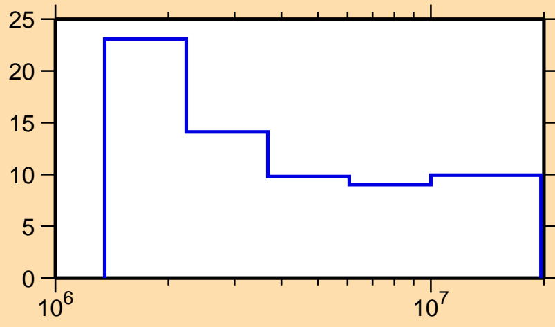
\Delta\sigma/\sigma vs. E for ^{204}\text{Bi}(n,n\text{nonel.})
