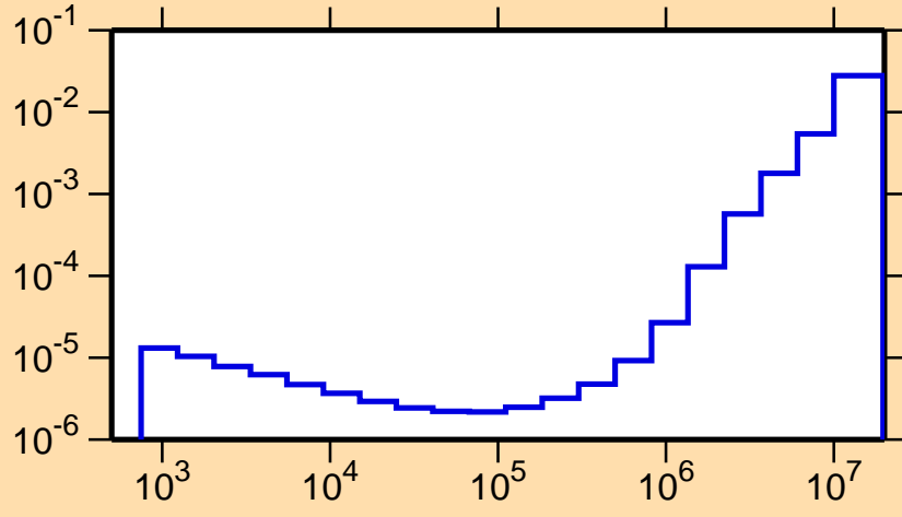
\sigma vs. E for ^{204}\text{Bi}(n,p)
