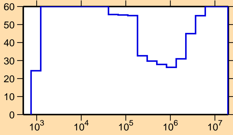
\Delta\sigma/\sigma vs. E for ^{204}\text{Bi}(n,\gamma)
