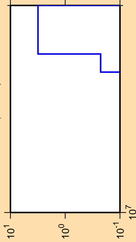
\Delta\sigma/\sigma vs. E for ^{205}\text{Bi}(n,3n\alpha)
