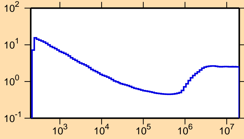
\sigma vs. E for ^{205}\text{Bi}(n,\text{nonel.})
