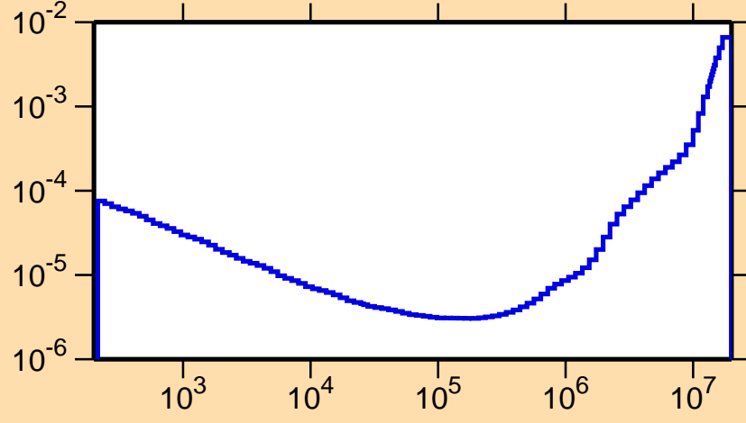
\sigma vs. E for ^{205}\text{Bi}(n,\alpha)
