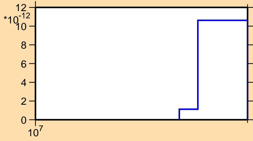
\sigma vs. E for ^{205}\text{Bi} (mt 45)
