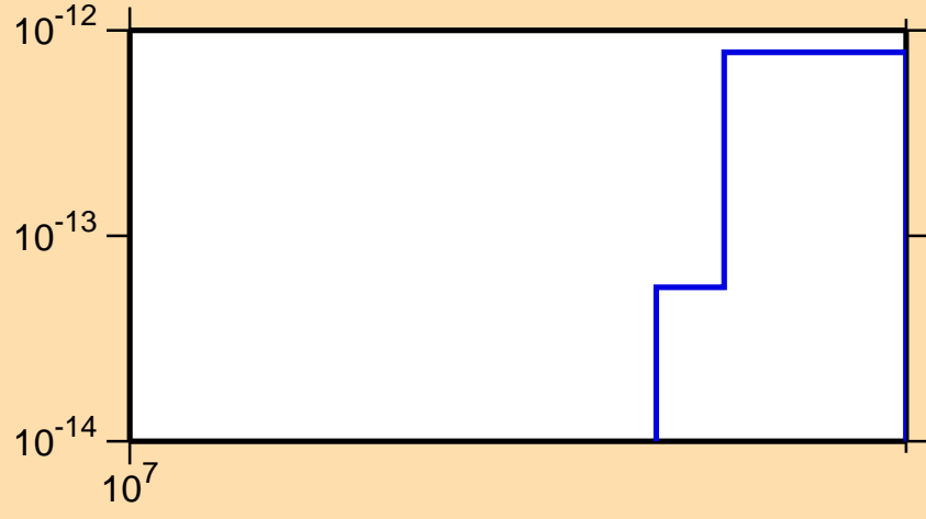
\sigma vs. E for ^{205}\text{Bi}(n,3n\alpha)
