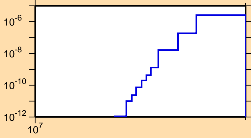
\sigma vs. E for ^{205}\text{Bi}(n,\text{nd})
