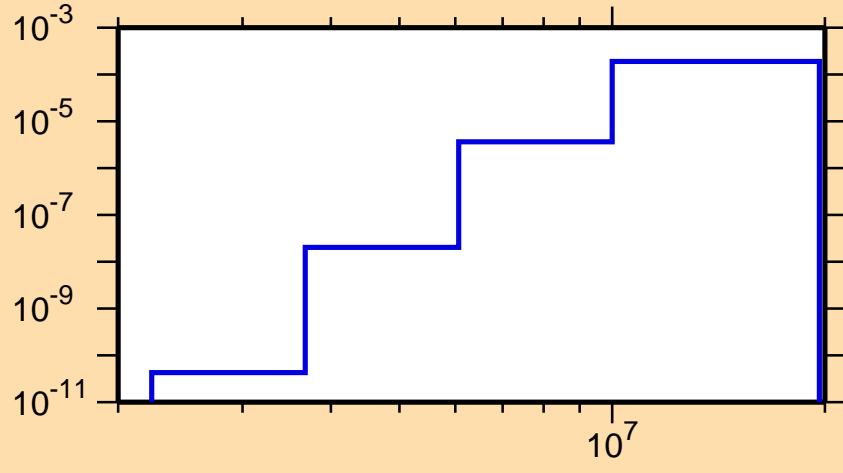
\sigma vs. E for ^{205}\text{Bi}(n,n\alpha)
