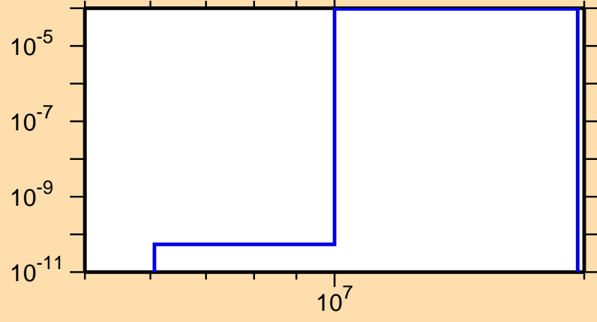
\sigma vs. E for ^{205}\text{Bi}(n,t)
