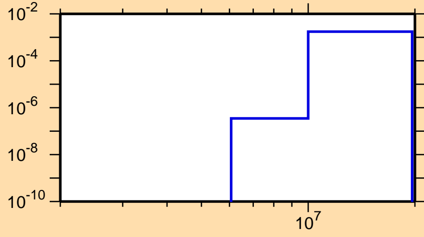
\sigma vs. E for ^{205}\text{Bi}(n,d)
