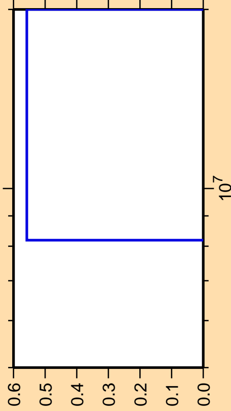
\Delta\sigma/\sigma vs. E for ^{205}\text{Bi}(\text{mt117})
