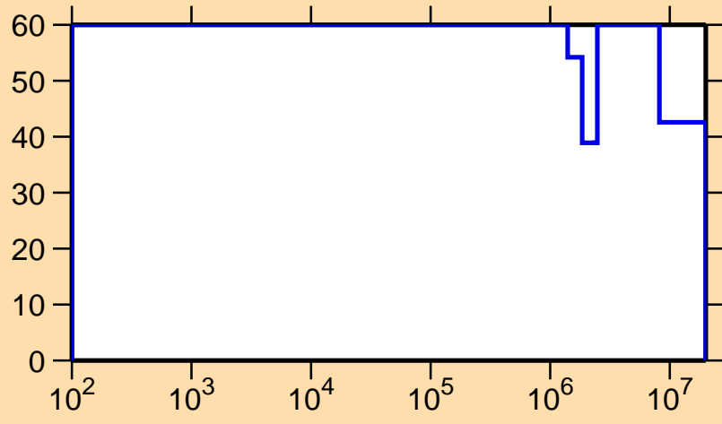
\Delta\sigma/\sigma vs. E for ^{205}\text{Bi}(n,p)
