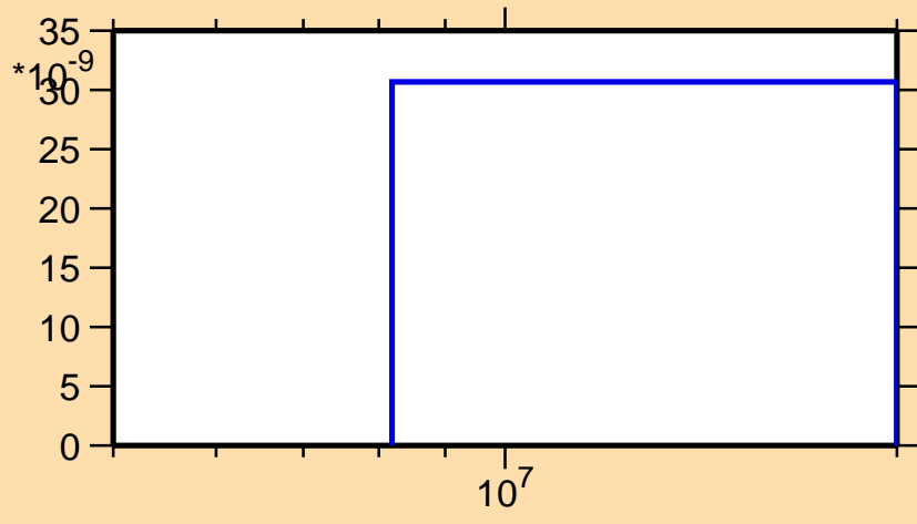
\sigma vs. E for ^{205}\text{Bi}(n,\text{nd})
