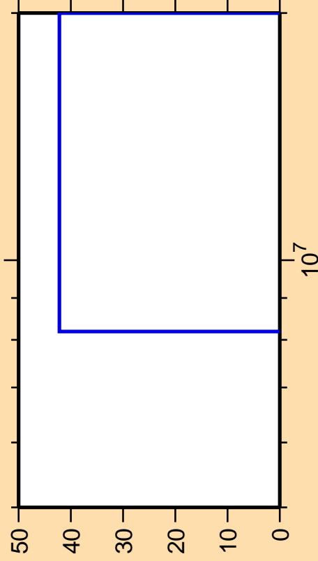
\Delta\sigma/\sigma vs. E for ^{205}\text{Bi}(n,n_1)
