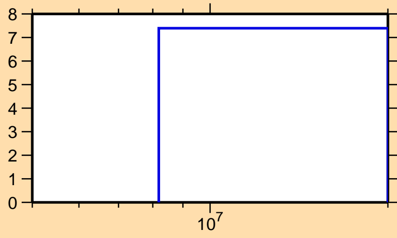
\Delta\sigma/\sigma vs. E for ^{205}\text{Bi}(n,\text{nonel.})
