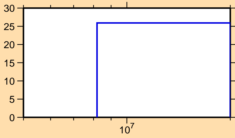
\Delta\sigma/\sigma vs. E for ^{205}\text{Bi}(n,2n)
