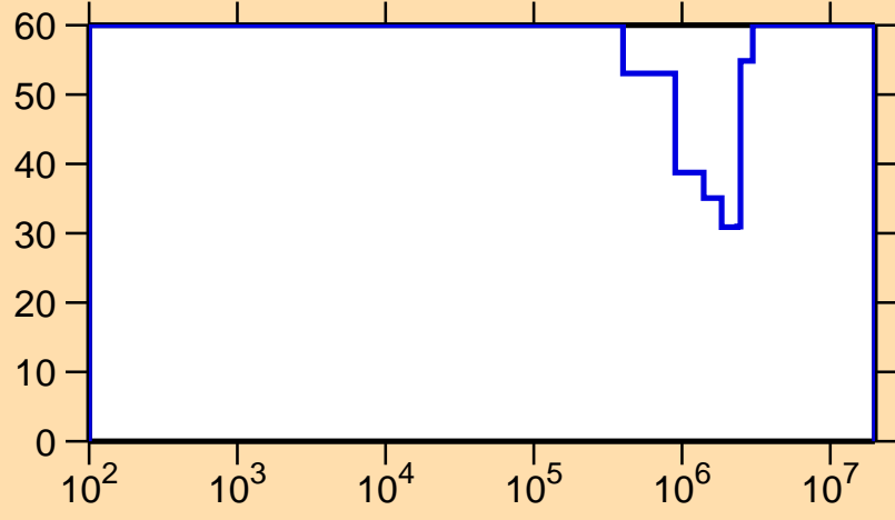
\Delta\sigma/\sigma vs. E for ^{205}\text{Bi}(n,\gamma)
