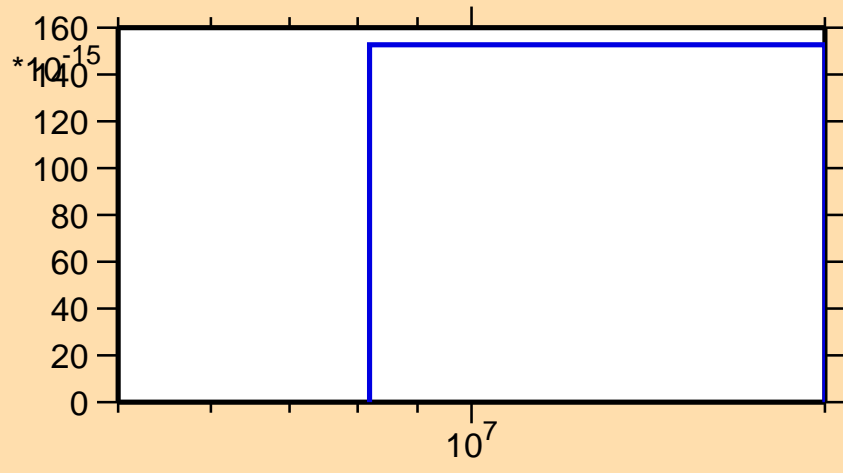
\sigma vs. E for ^{205}\text{Bi} (mt 45)
