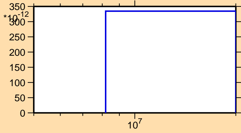
\sigma vs. E for ^{205}\text{Bi}(n,\text{He3})
