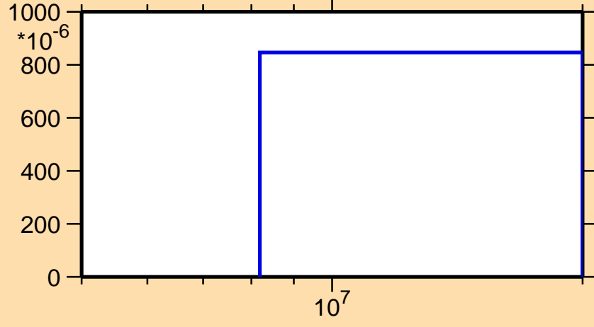
\sigma vs. E for ^{205}\text{Bi}(n,3n)
