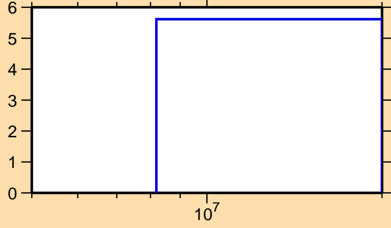
\Delta\sigma/\sigma vs. E for ^{205}\text{Bi}(n,\text{tot.})
