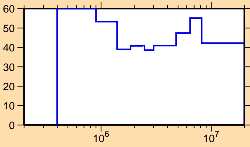
\Delta\sigma/\sigma vs. E for ^{205}\text{Bi}(n,n_1)
