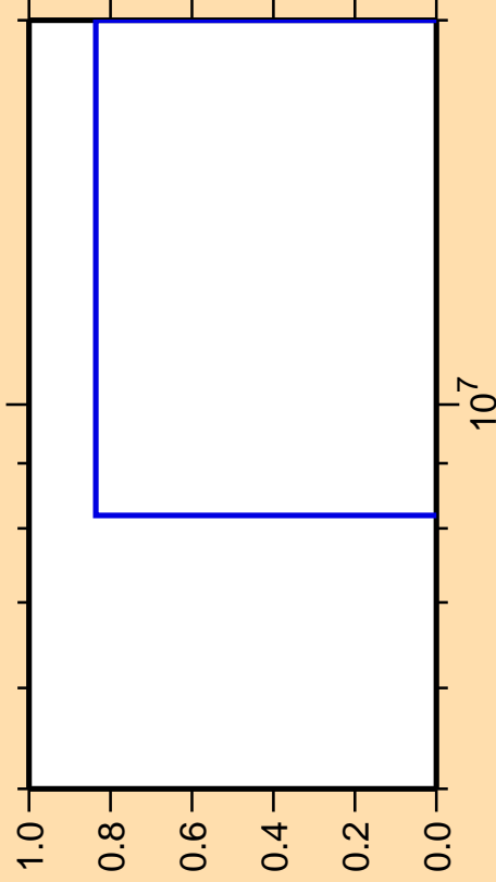
\Delta\sigma/\sigma vs. E for ^{205}\text{Bi} (mt 45)
