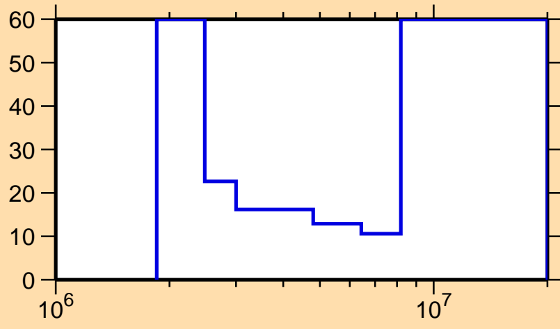
\Delta\sigma/\sigma vs. E for ^{205}\text{Bi}(n,n\text{cont.})
