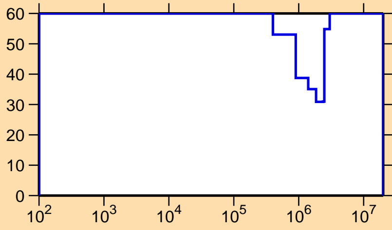
\Delta\sigma/\sigma vs. E for ^{205}\text{Bi}(n,\gamma)
