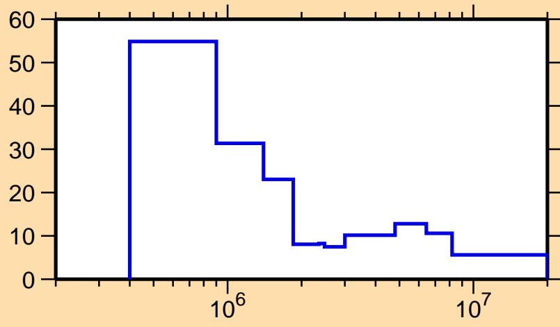
\Delta\sigma/\sigma vs. E for ^{205}\text{Bi}(n,\text{tot.})
