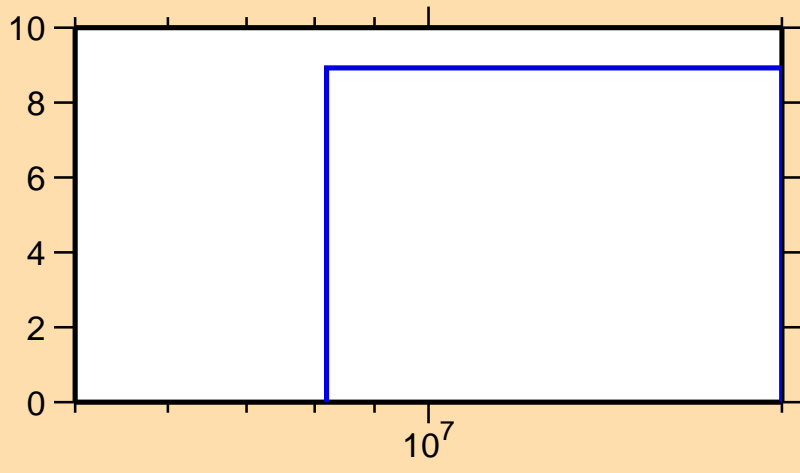
\Delta\sigma/\sigma vs. E for ^{205}\text{Bi}(n,\text{el.})
