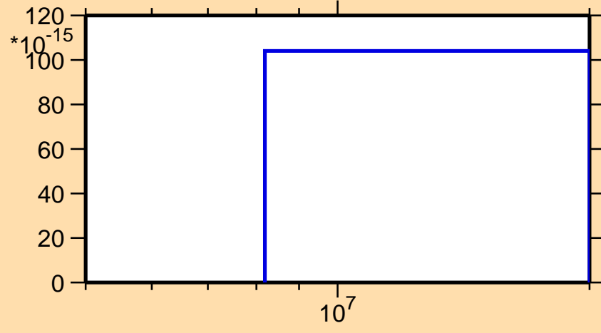
\sigma vs. E for ^{205}\text{Bi}(\text{mt117})
