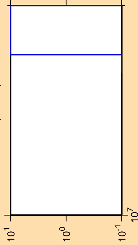
\Delta\sigma/\sigma vs. E for ^{206}\text{Bi}(n,3n\alpha)
