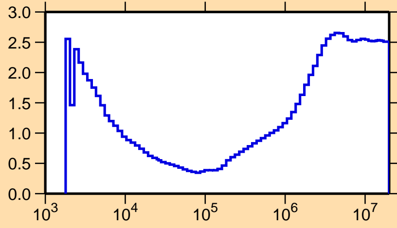
\sigma vs. E for ^{206}\text{Bi}(n,\text{nonel.})
