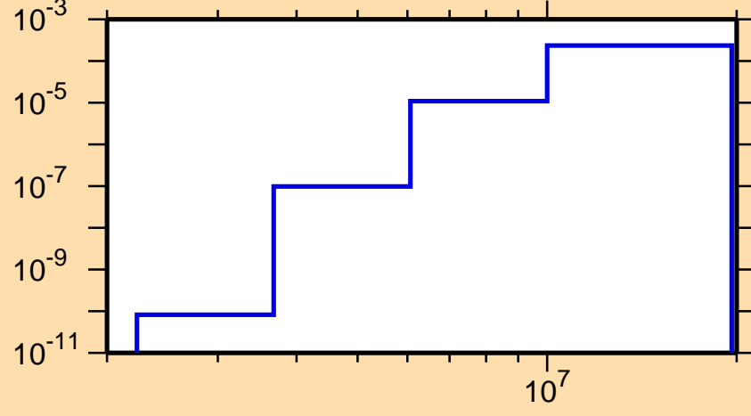
\sigma vs. E for ^{206}\text{Bi}(n,n\alpha)
