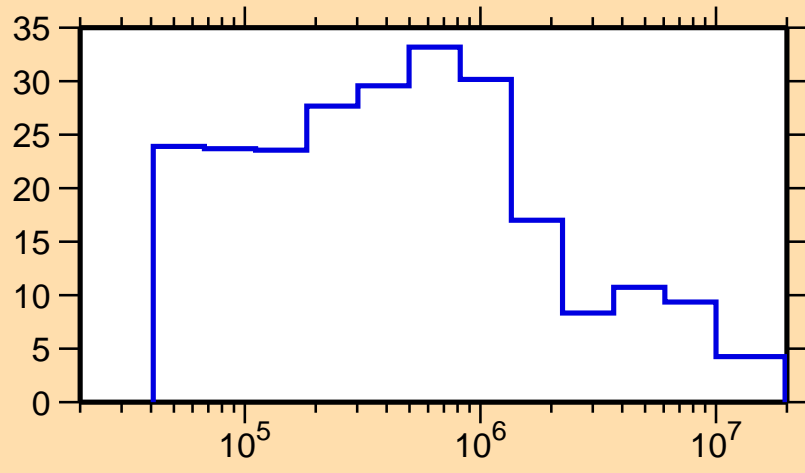
\Delta\sigma/\sigma vs. E for ^{206}\text{Bi}(n,\text{tot.})
