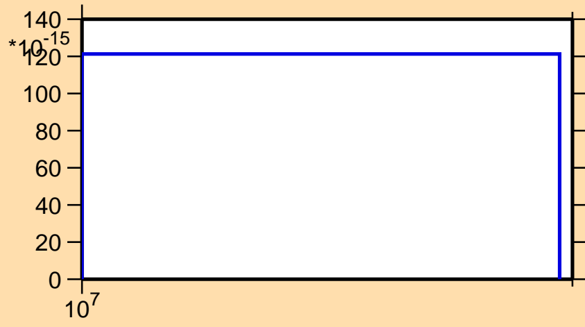
\sigma vs. E for ^{206}\text{Bi}(\text{mt117})
