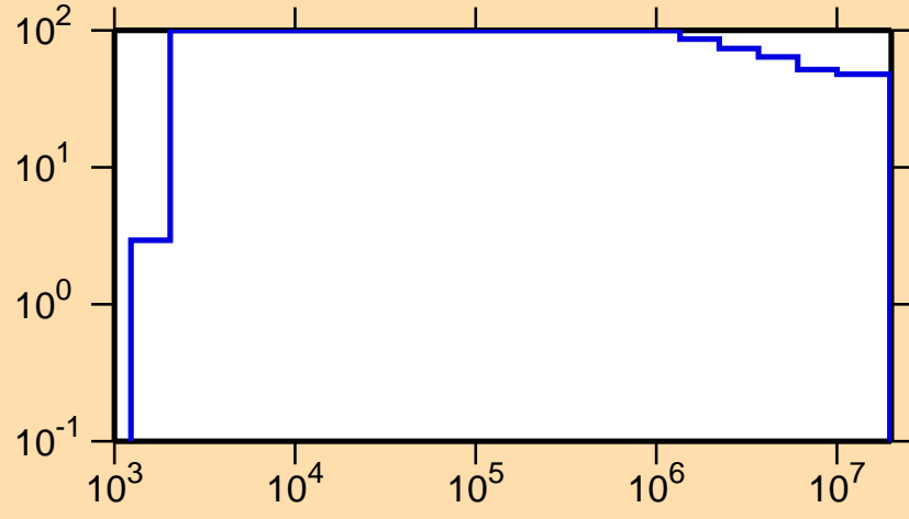
\Delta\sigma/\sigma vs. E for ^{206}\text{Bi}(n,p)
