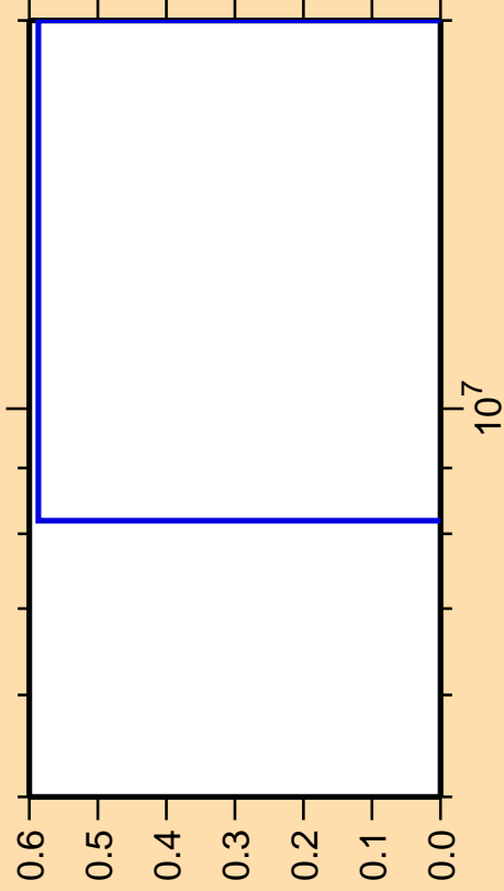
\Delta\sigma/\sigma vs. E for ^{206}\text{Bi}(\text{mt117})
