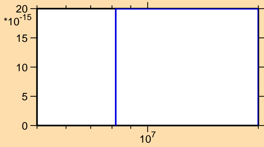
\sigma vs. E for ^{206}\text{Bi}(n,3n\alpha)
