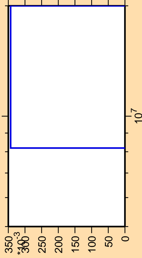
\Delta\sigma/\sigma vs. E for ^{206}\text{Bi} (mt 45)
