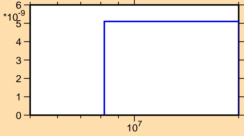
\sigma vs. E for ^{206}\text{Bi}(n,nt)
