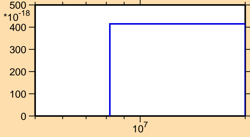
\sigma vs. E for ^{206}\text{Bi} (mt 34)
