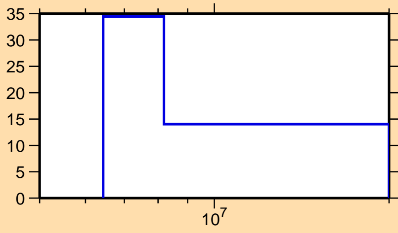
\Delta\sigma/\sigma vs. E for ^{206}\text{Bi}(n,2n)
