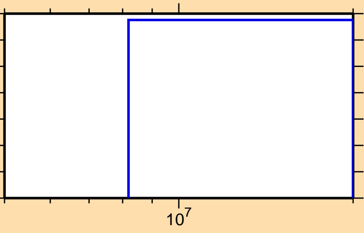
\sigma vs. E for ^{206}\text{Bi}(n,\text{He3})
