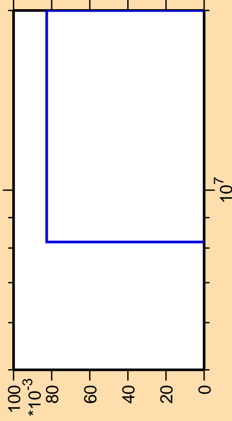
\Delta\sigma/\sigma vs. E for ^{206}\text{Bi}(n,3n\alpha)
