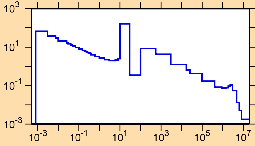
\sigma vs. E for ^{206}\text{Bi}(n,\gamma)
