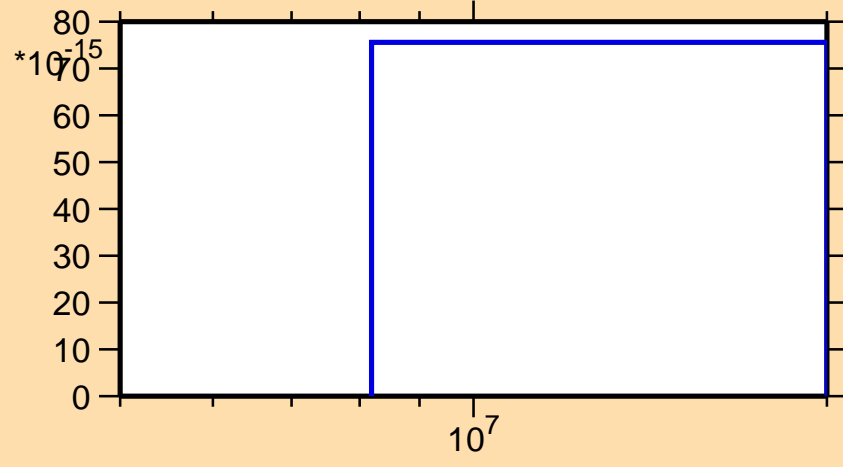
\sigma vs. E for ^{206}\text{Bi} (mt 45)
