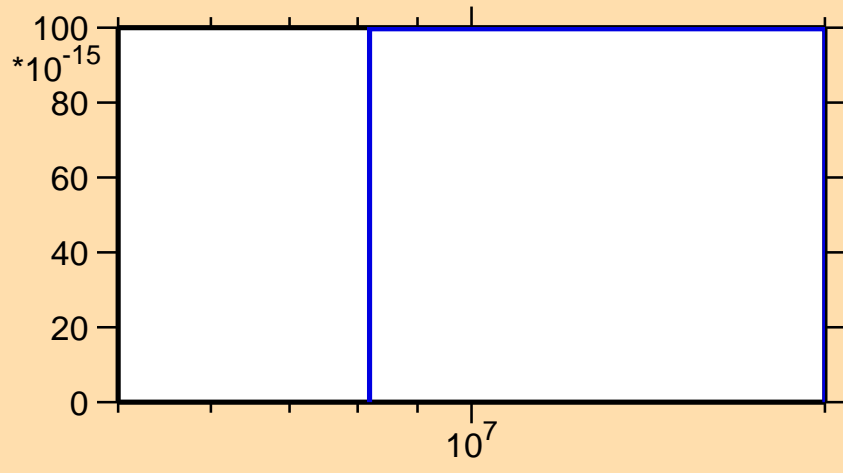
\sigma vs. E for ^{206}\text{Bi}(\text{mt117})
