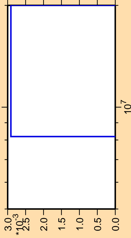
\Delta\sigma/\sigma vs. E for ^{206}\text{Bi} (mt 34)
