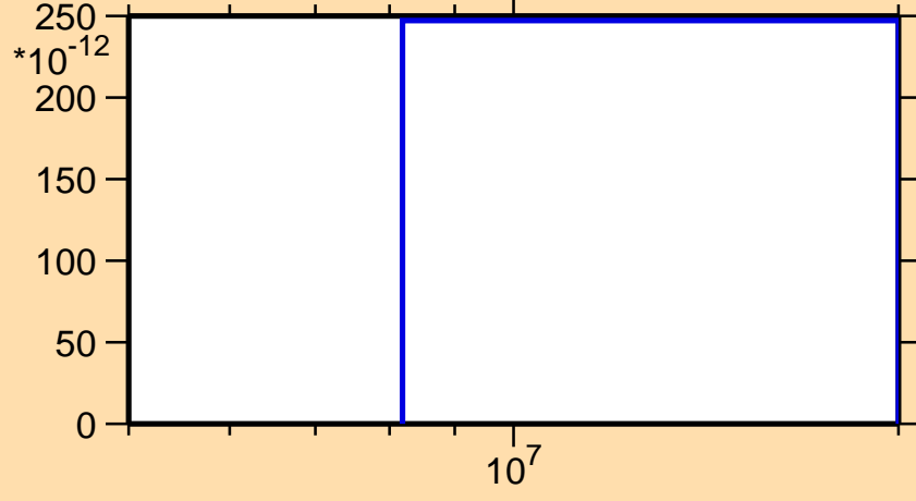
\sigma vs. E for ^{206}\text{Bi}(n,p\alpha)
