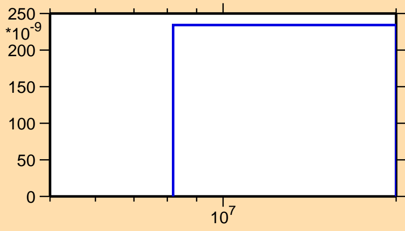
\sigma vs. E for ^{206}\text{Bi}(n,\text{nd})
