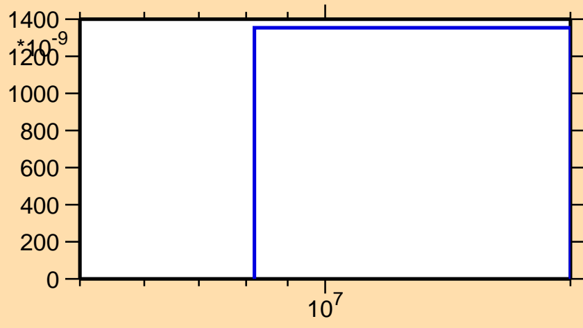
\sigma vs. E for ^{206}\text{Bi}(n,2n\alpha)
