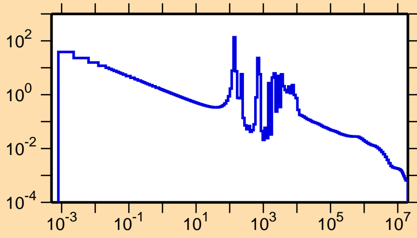
\sigma vs. E for ^{207}\text{Bi}(n,\gamma)
