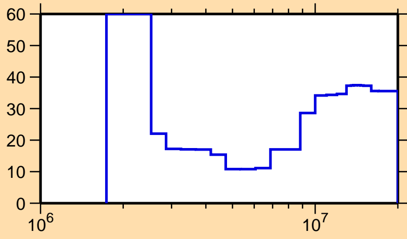
\Delta\sigma/\sigma vs. E for ^{207}\text{Bi}(n,n\text{cont.})
