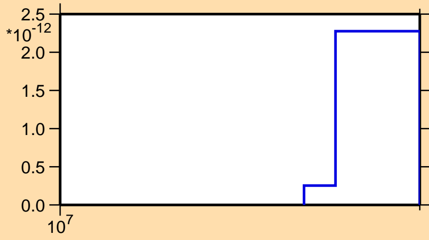
\sigma vs. E for ^{207}\text{Bi}(\text{mt117})
