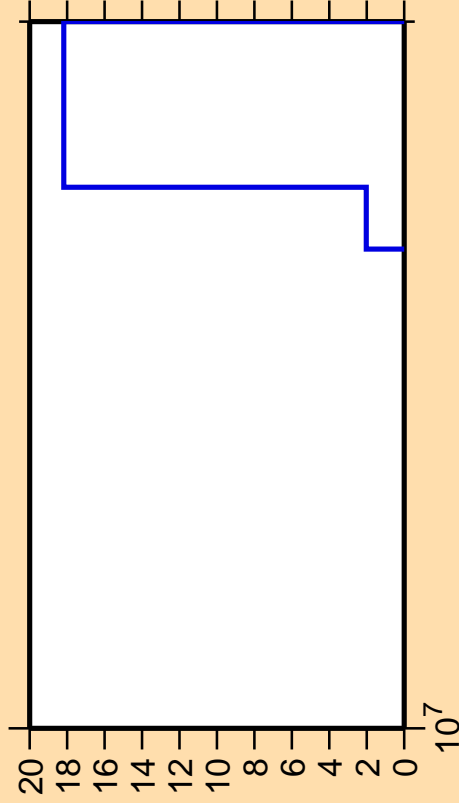
\Delta\sigma/\sigma vs. E for ^{207}\text{Bi}(\text{mt117})
