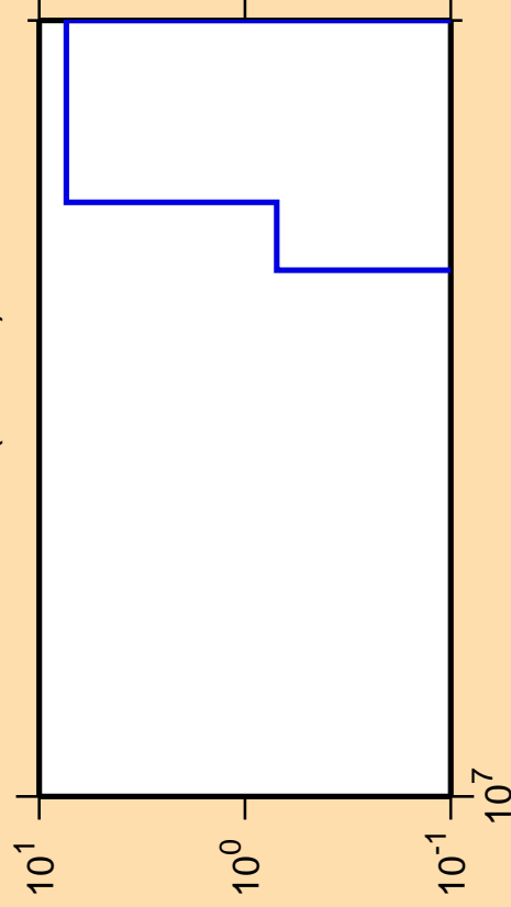
\Delta\sigma/\sigma vs. E for ^{207}\text{Bi} (mt 45)
