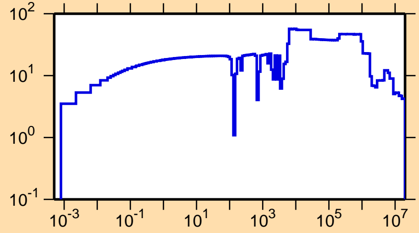
\Delta\sigma/\sigma vs. E for ^{207}\text{Bi}(n,\text{tot.})
