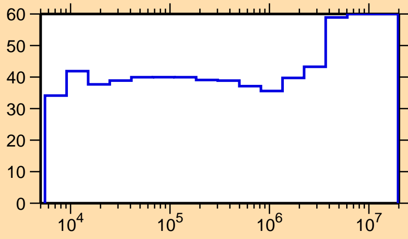
\Delta\sigma/\sigma vs. E for ^{207}\text{Bi}(n,\gamma)
