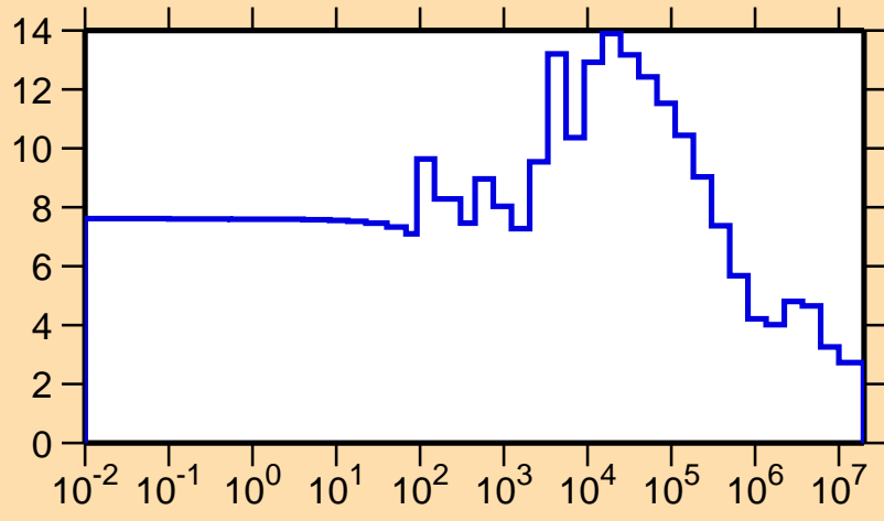
\sigma vs. E for ^{207}\text{Bi}(n,\text{el.})
