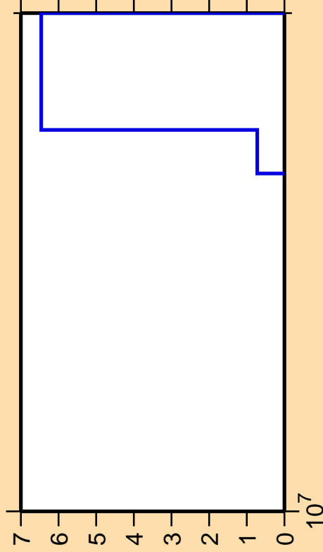
\Delta\sigma/\sigma vs. E for ^{208}\text{Bi}(\text{mt117})
