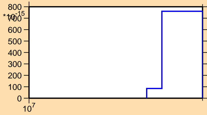
\sigma vs. E for ^{208}\text{Bi}(\text{mt117})
