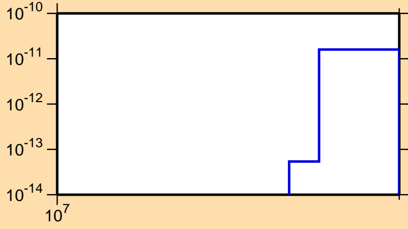
\sigma vs. E for ^{208}\text{Bi}(n,3n\alpha)
