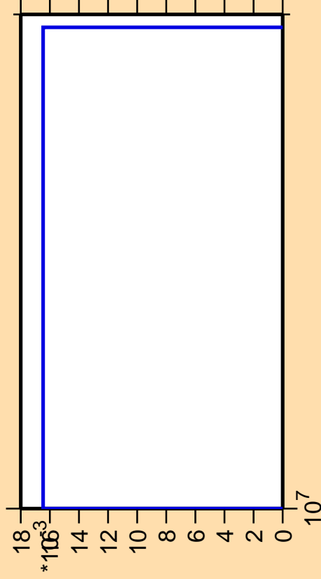
\Delta\sigma/\sigma vs. E for ^{208}\text{Bi} (mt 45)
