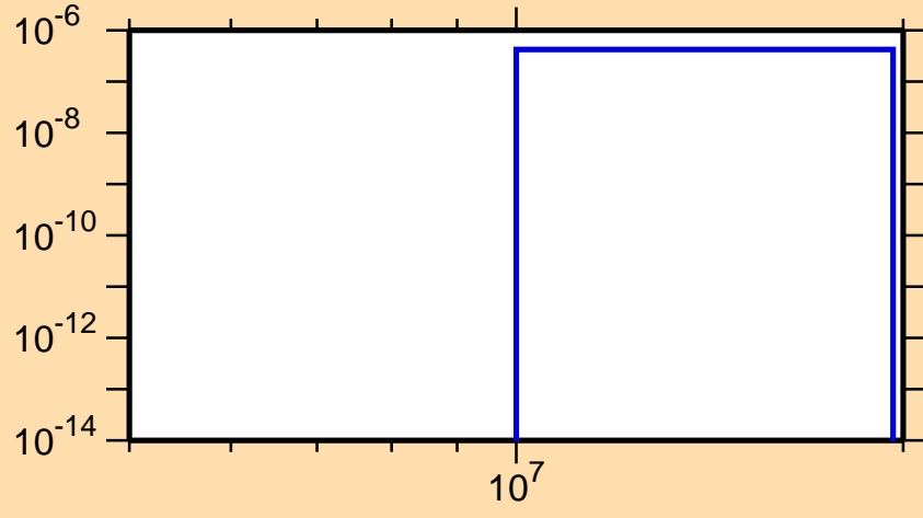
\sigma vs. E for ^{208}\text{Bi}(n,nd)
