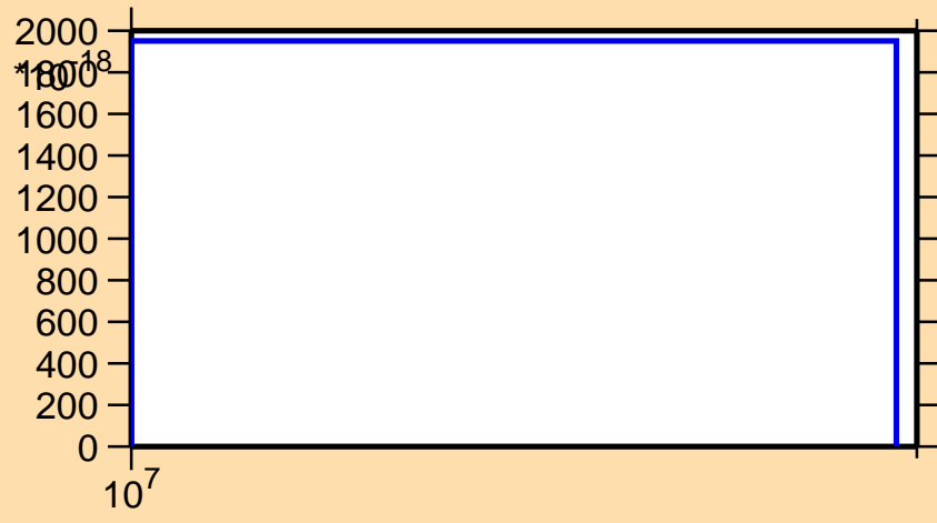
\sigma vs. E for ^{208}\text{Bi} (mt 45)
