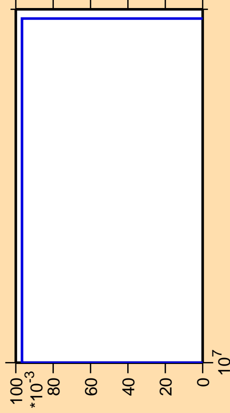
\Delta\sigma/\sigma vs. E for ^{208}\text{Bi}(\text{mt117})
